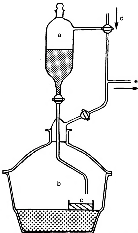
FIGURE 1.—Impregnation apparatus: a , vessel containing resin; b , desiccator containing anhydrous \text{CaCl}_2 and the sample ( c ) for impregnation; d , inlet for air into a and b ; e , suction by water pump via a silica gel vessel inserted into the vacuum line.
