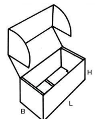
FEFCO 0471
