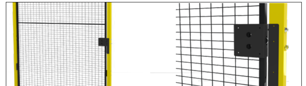
T10-32 Fittings, Schmersal AZM200 hingedoor, right/left
