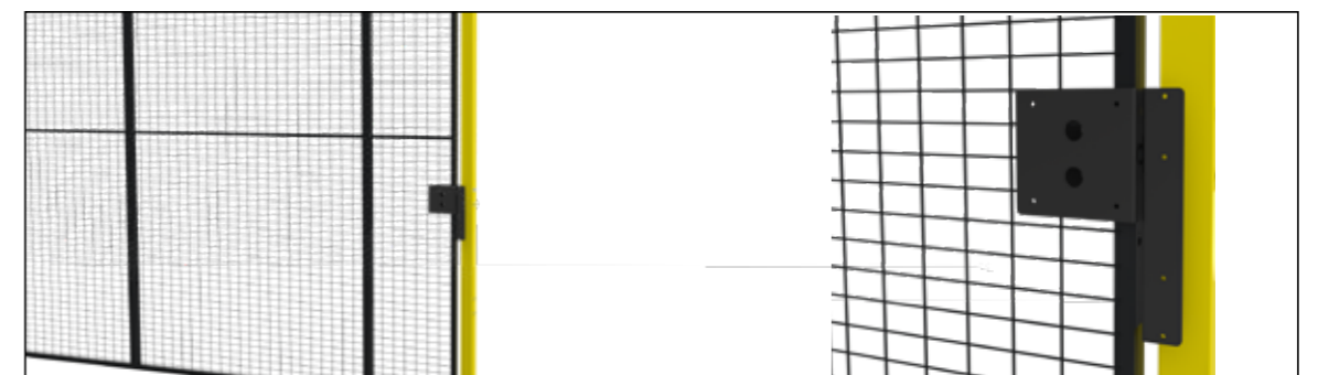
T10-32 Fittings, Schmersal AZM200 slidingdoor, right/left
