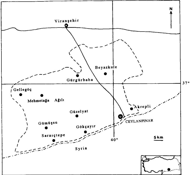
Fig. 1. Geographic map of study area.
