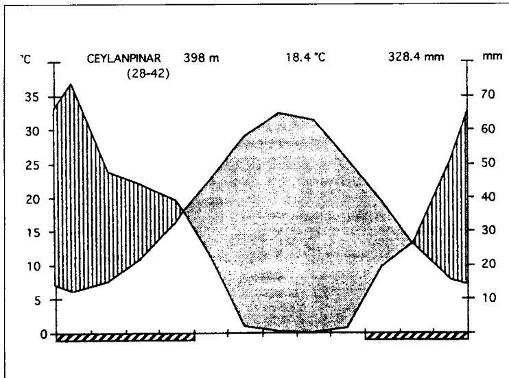
Fig. 2. Ombrothermic diagram of Ceylanpınar.
