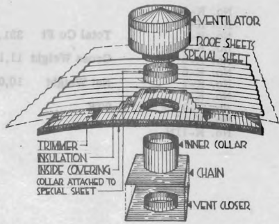
VENTILATOR CONSTRUCTION
