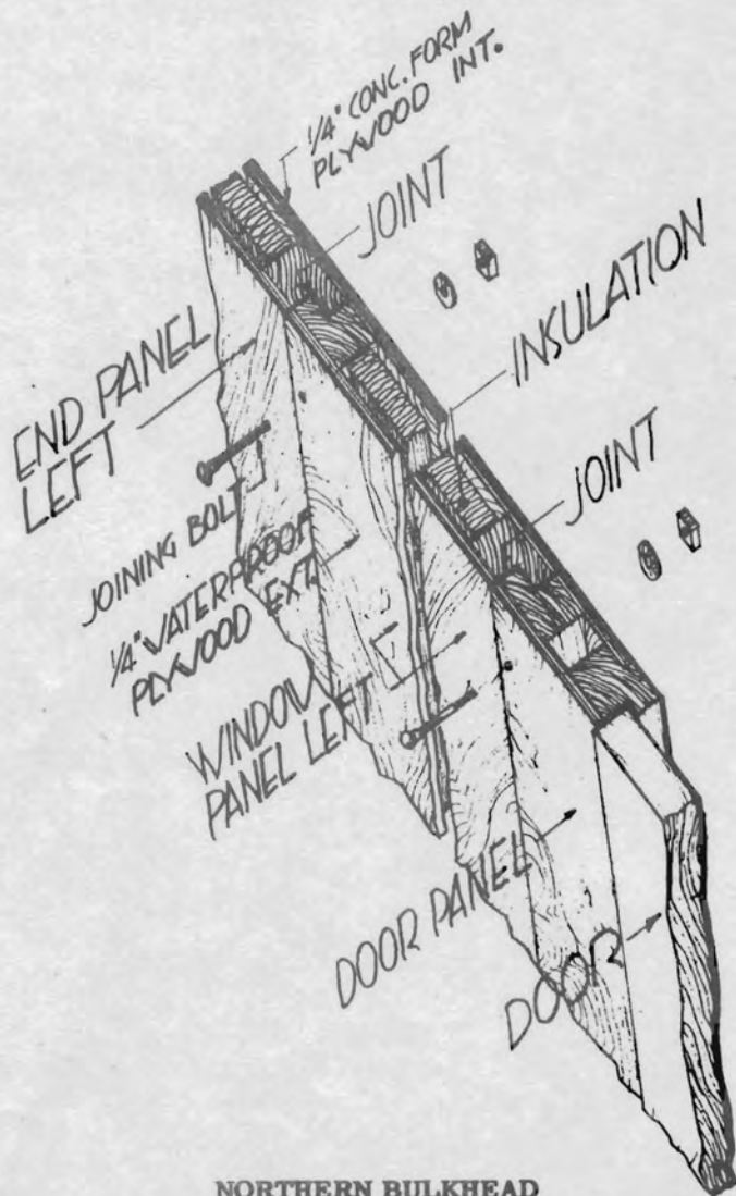
NORTHERN BULKHEAD
