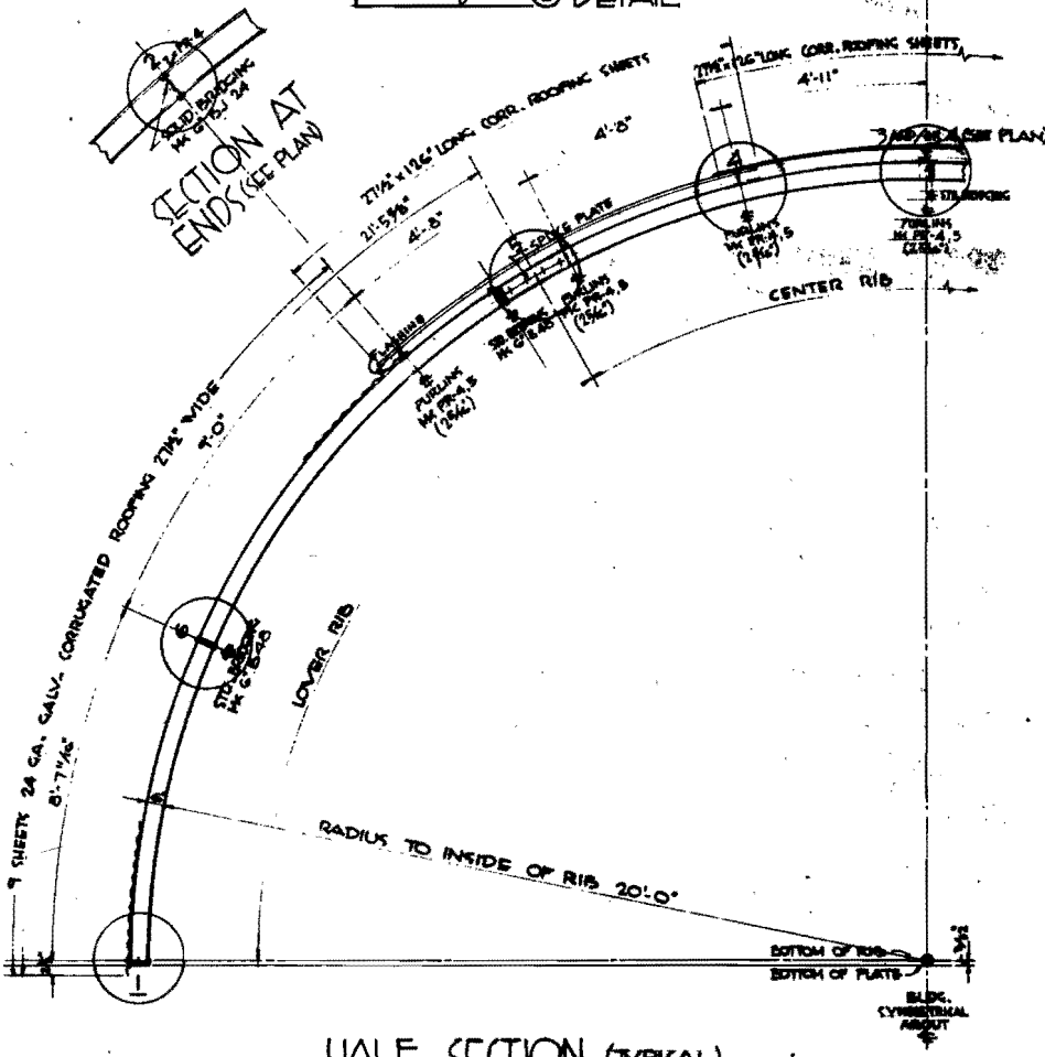
HALF SECTION (TYPICAL)
