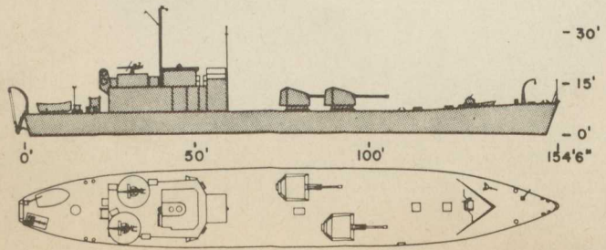
LSSL 3. BRITISH LCG (M) CLASS
