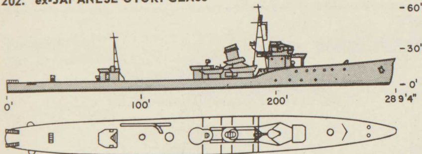
202. ex-JAPANESE OTORI CLASS
