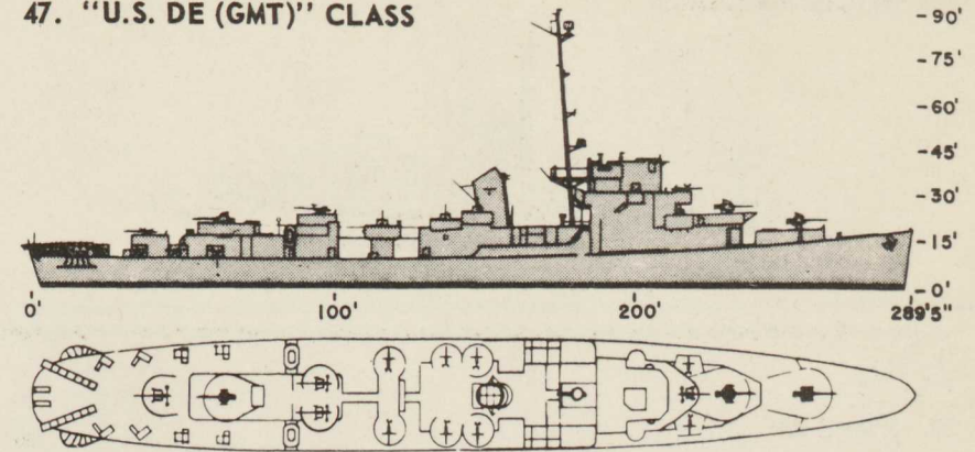
47. "U.S. DE (GMT)" CLASS
