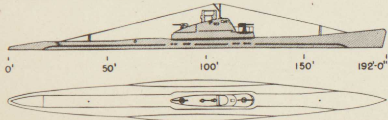
247. "SHCH III" CLASS
