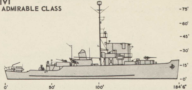
CMC 63. YUNG CHING
