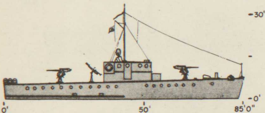
216. "MO I" CLASS
