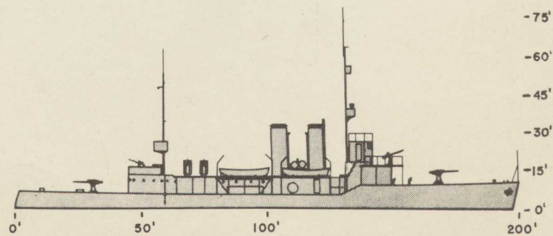
PG 9. MIN CHUAN
