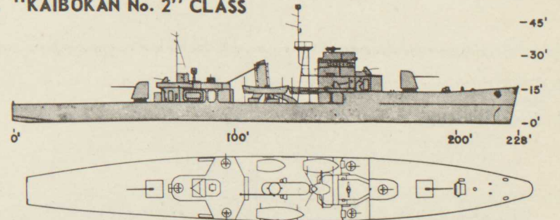
14. "KAIBOKAN No. 2" CLASS
