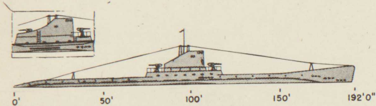
246. "SHCH II" CLASS. Insert shows conning tower variation.
