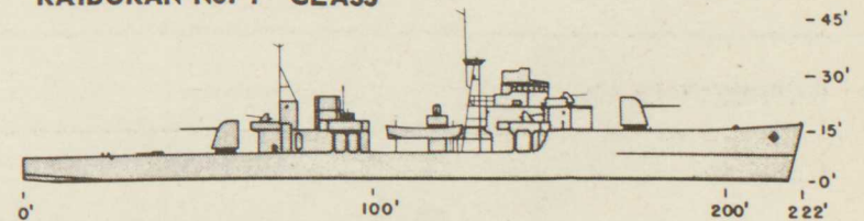
15. "KAIBOKAN No. 1" CLASS
