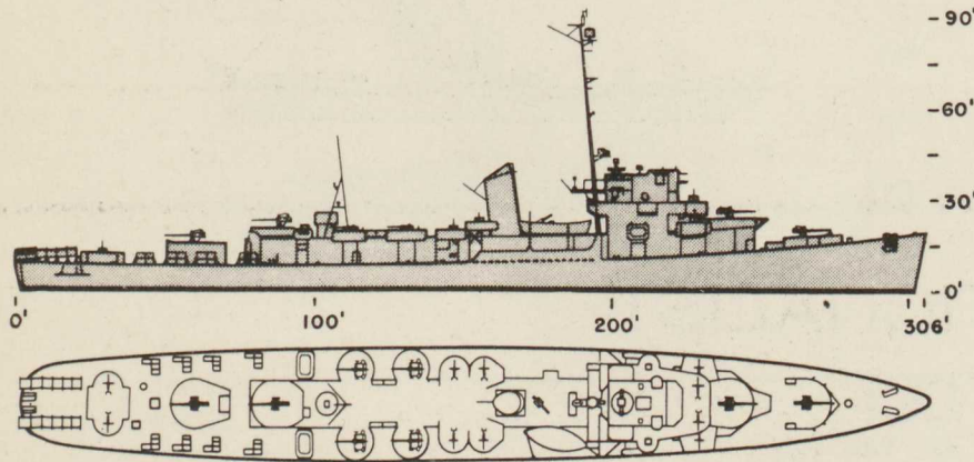
45. "U.S. DE (DET)" CLASS
