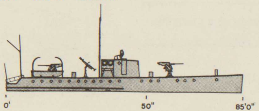
220. "MO IV" CLASS
