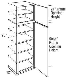
U129312-U249312 L or R
