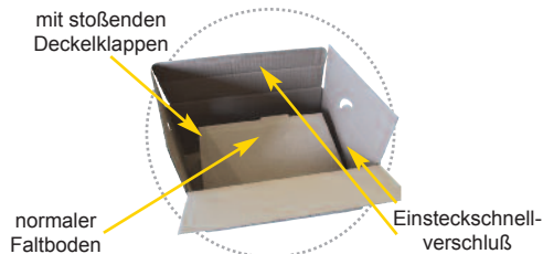
Fefco 0711
