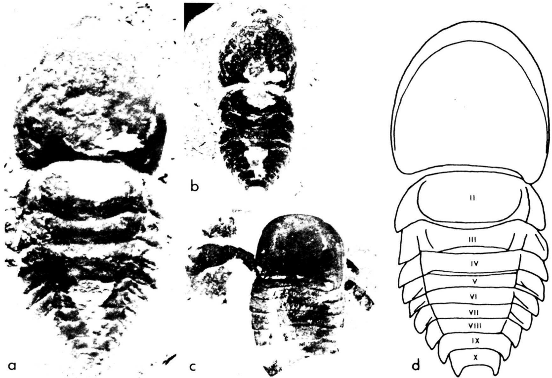
TEXT-FIG. 3. a, b, d , Pasternakevia podolica gen. et sp. nov., No. 35611, holotype and only known specimen; upper part of Ustye Suite, Bagovytsa Horizon (middle Ludlow), near Velyka Slobidka, Ukraine, USSR; a , dorsal view in low-angle light, \times 3.0 ; b , dorsal view in high-angle light, \times 1.5 ; d , outline drawing of specimen showing main features and tergite numbers, \times 3.0 . c , Baltoeurypterus tetragonophthalmus (Fischer, 1839), No. 35612, from same horizon and locality as Pasternakevia , \times 1 .
