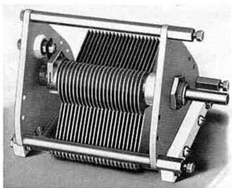
This TYPE 539-TA Condenser is of interest because the entire rotor assembly (as well as the stator) is insulated from the end plates
