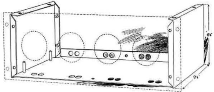
Type 661-L End- and Base-Plate Assembly For 19 x 7-inch Panels
