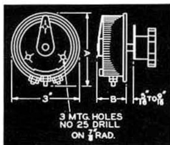
Standard 3-hole mounting method for rheostat-potentiometers
