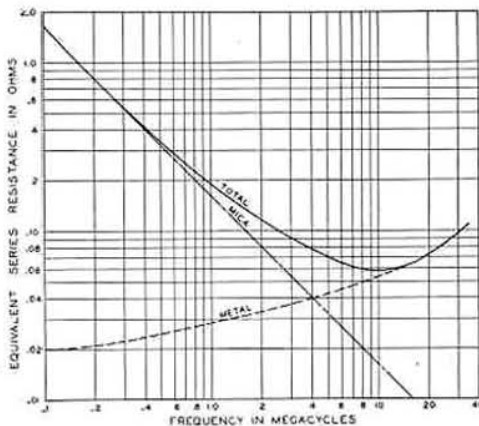
Equivalent-resistance-versus-frequency characteristic of a typical TYPE 505 Condenser
