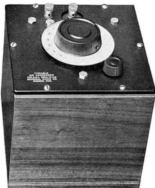
The TYPE 246 Condenser is like the TYPE 222 Precision Condenser, but it has no micrometer drive
