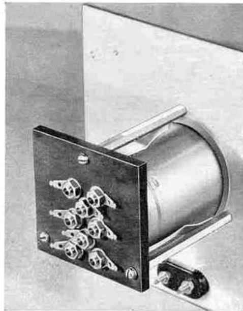
The complete shielded inductor mounts in this manner on a unit panel. The three springs on the TYPE 661-P10 Jack Base guide the inductor into place.
