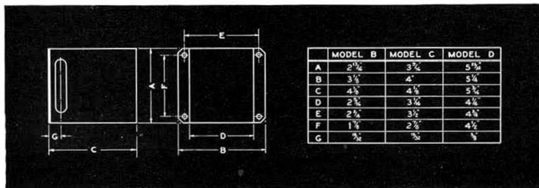
Dimensions for standard general audio transformer-mounting cases
