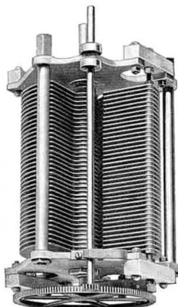
The TYPE 246 Condenser is like the TYPE 222 Precision Condenser, but it has no micrometer drive
