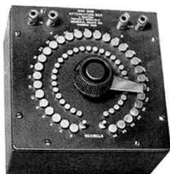
The TYPE 529 Attenuation Box is made as an L-type section which maintains constant impedance at the 1-2 terminals
