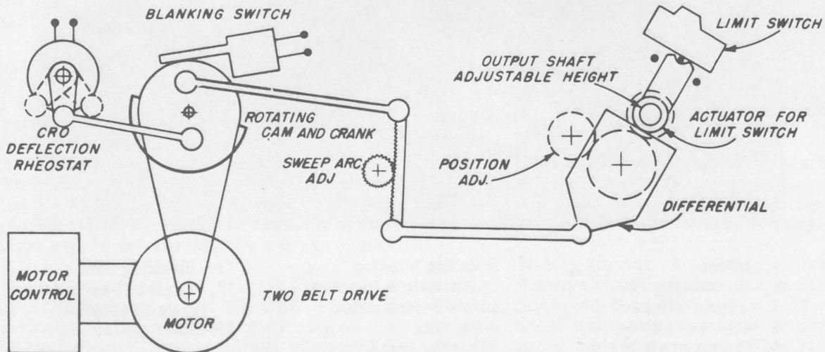
Figure 2. Elementary Mechanical Diagram.
