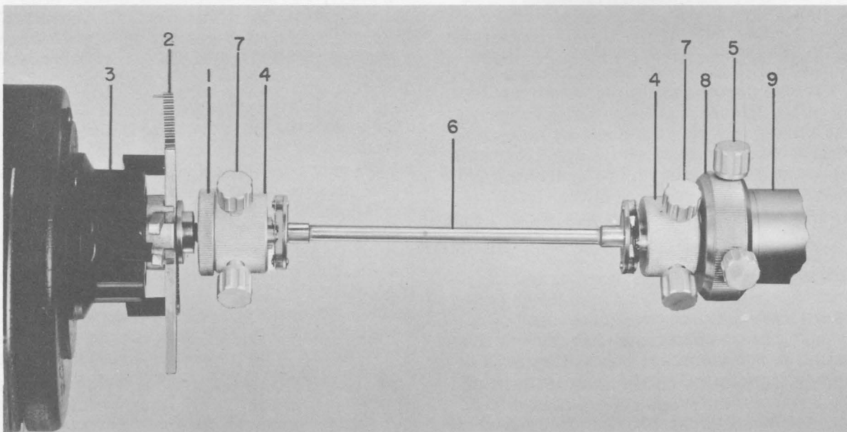
Figure 7. Coupling Attachments.
