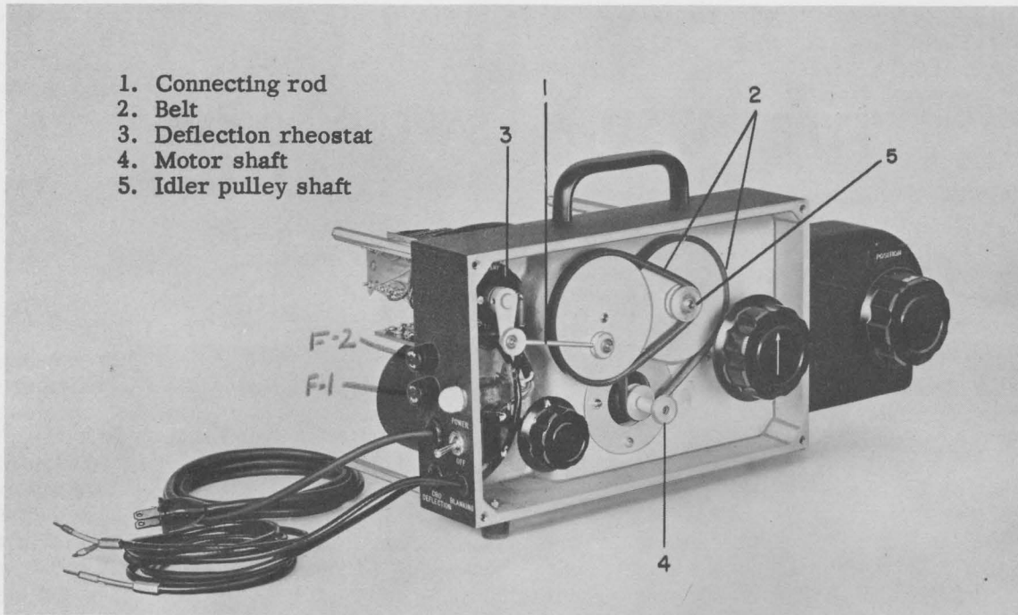
Figure 3. Front Interior View.
