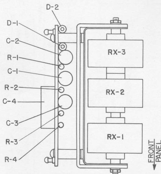
Figure 9. Electrical Components.
