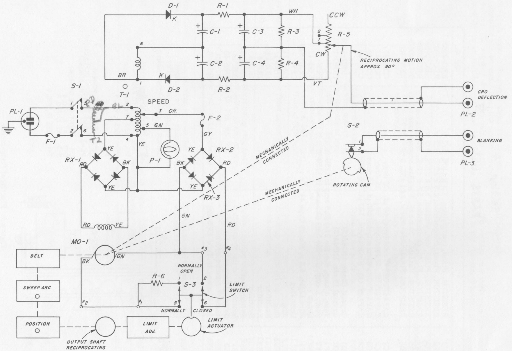
Figure 10. Schematic Wiring Diagram.
