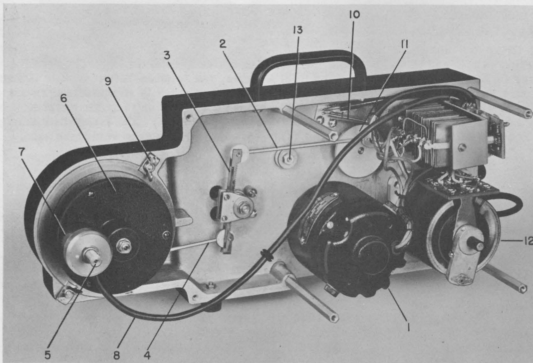
Figure 3. Front Interior View.
