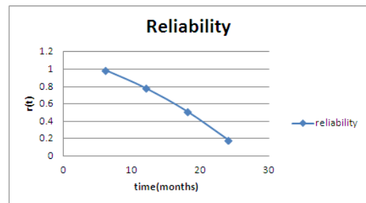
Fig.6: Reliability Graph for pulper using Parametric method
