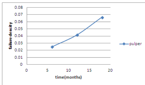
Fig.3: Failure density graph for pulper
