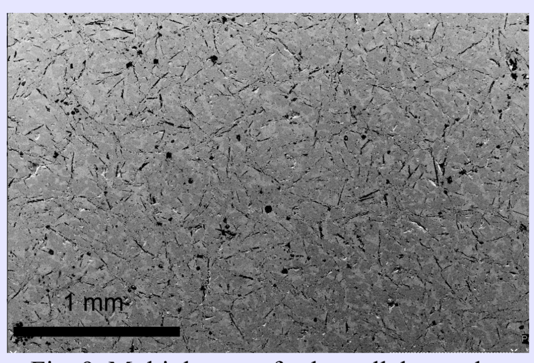
Fig. 9. Multiple sets of subparallel, mostly open fractures in iron silicide matrix.
