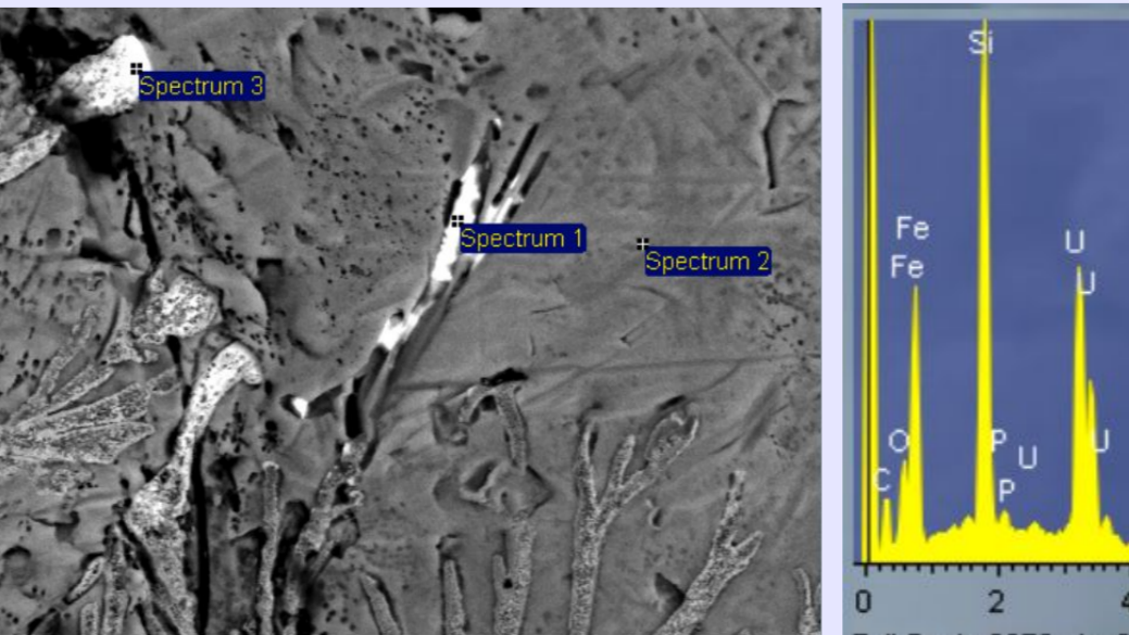
Fig. 16. Iron silicide with significant uranium peak in spectrum 1 (to the right). Spectrum 2 shows uranium and mostly zirconium (similar to Fig. 5), spectrum 3 more or less pure iron silicide. Spectra 2, 3 not shown here.
