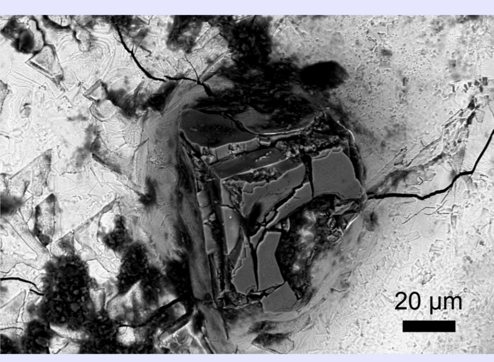
Fig. 10. Strongly fractured titanium carbide crystal in iron silicide matrix. Note the open, tensile fractures pointing to dynamic (shock?) spallation fracturing.
