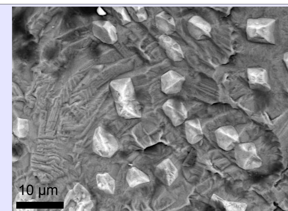
Fig. 5. Zircon crystals in iron silicide matrix. The white tips on the crystals have been shown to be uranium.
