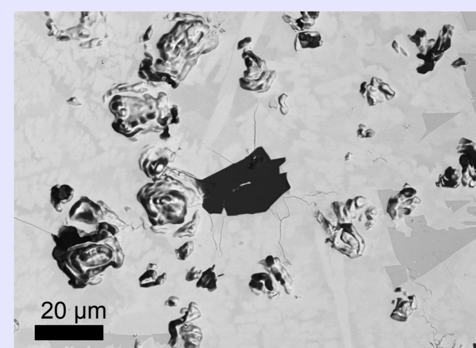
Fig. 8. Peculiar ornate structures in the iron silicide matrix lacking a conclusive explanation. Possibly spotty melting of the matrix.
