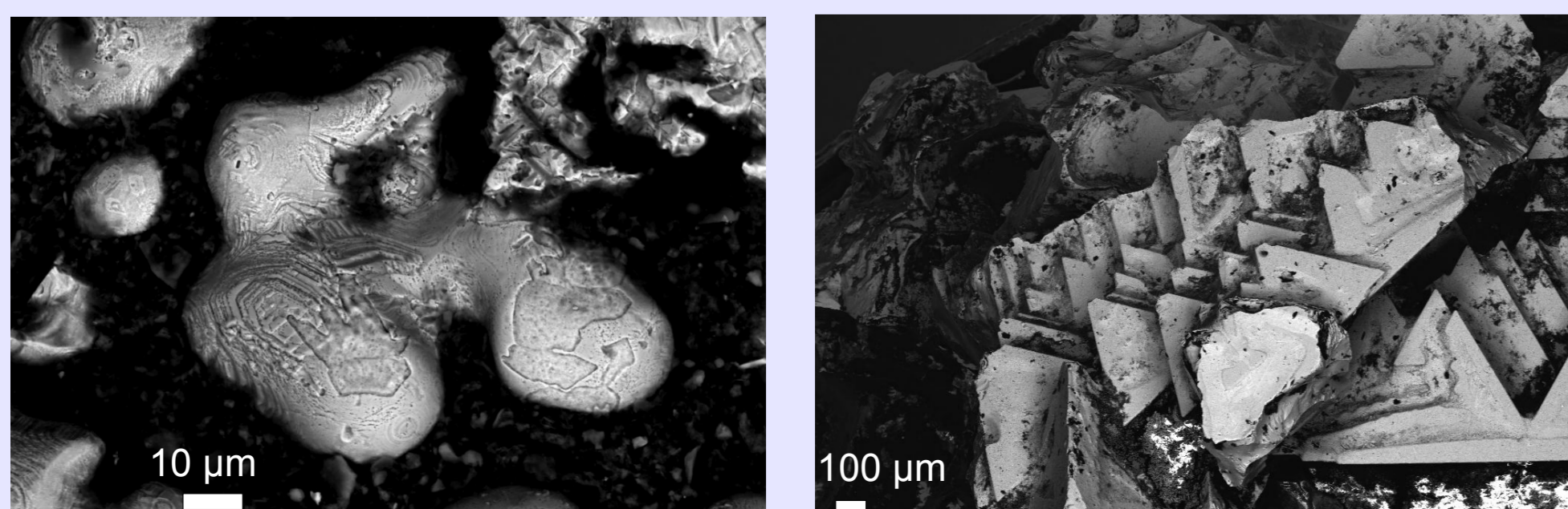
Fig. 4. Amoeba-like and pyramidal-shaped iron silicide in widely unstructured iron silicide.
