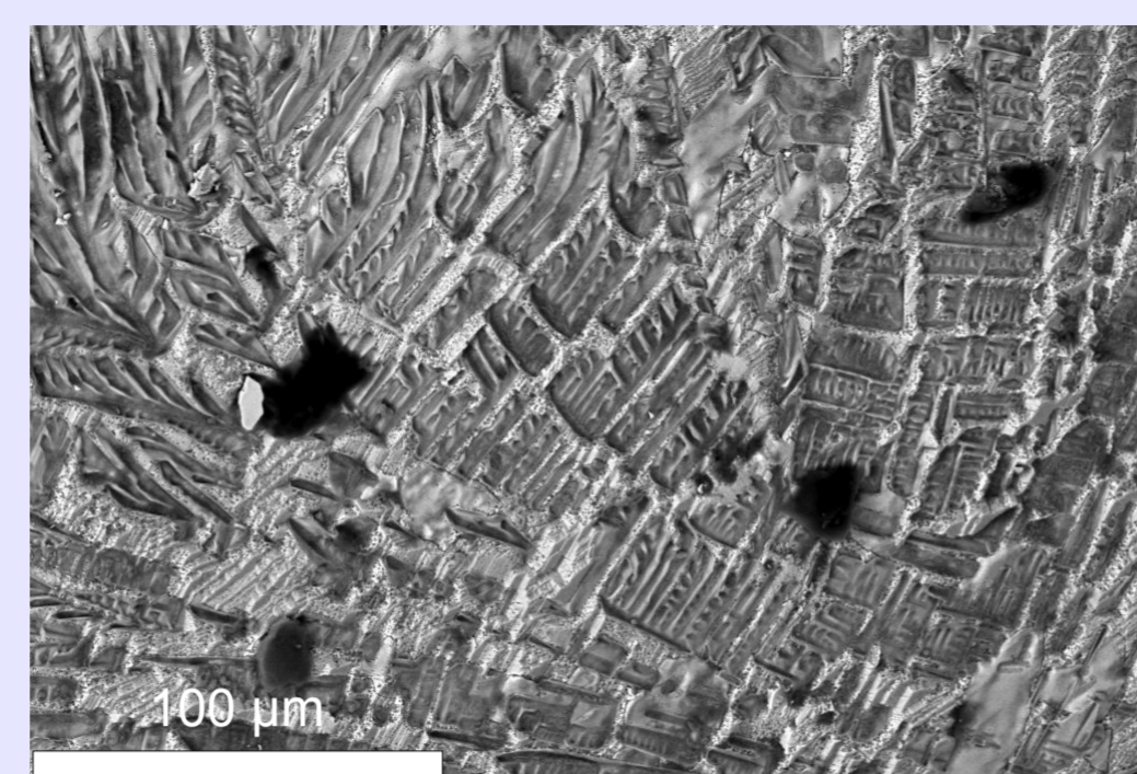
Fig. 7. Zirconium (zircon or/and baddeleyite) possible exsolution lamellae in iron silicide.
