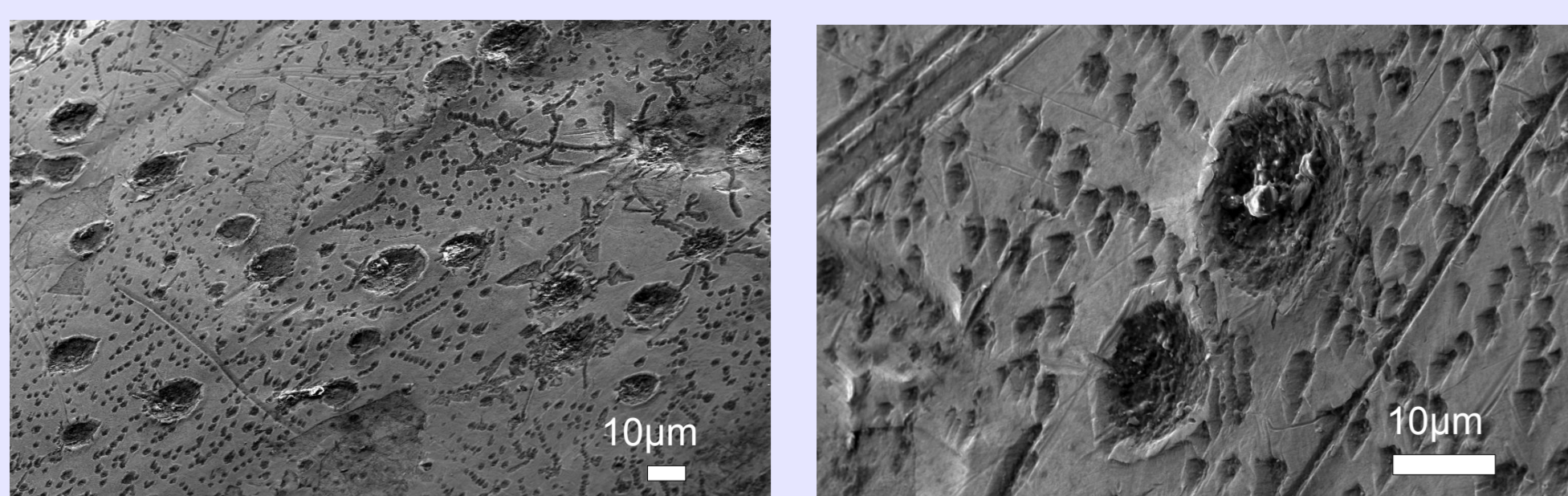
Fig. 3. Rimmed micro-craters on the surface of an iron silicide particle and two craters in more detail. The many angular pits could be imprints of zircon crystals now removed (see Fig. 5).
