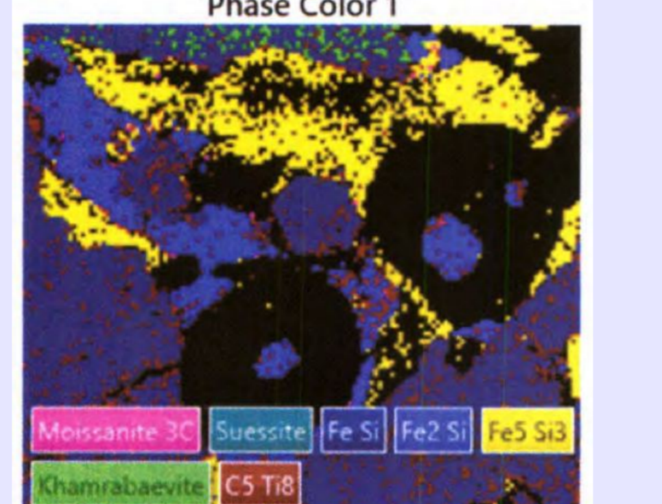
Fig. 14. Phase diagram for moissanite and titanium carbide phases in iron silicide matrix. Suessite is represented by only few counts. The black areas seem to be a calcium silicate near to wollastonite-1T without matching it and possibly being one of the several CaSiO 3 polymorphs.
