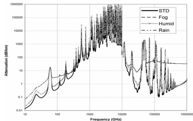
FIGURE 4. Atmospheric attenuation for horizontal path links at sea level for different weather conditions [6].
