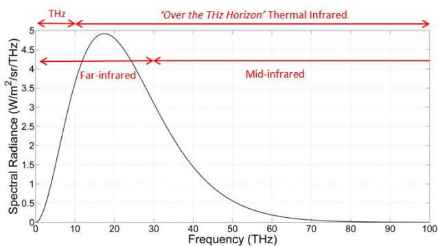
FIGURE 1. Calculated Planckian spectrum for a blackbody radiator at 296 K as a function of frequency. (Spectral bands defined here are overlaid in red).
