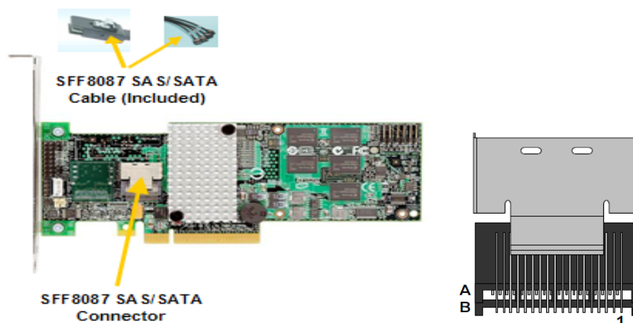
Figure 5. SAS/SATA Connectors
