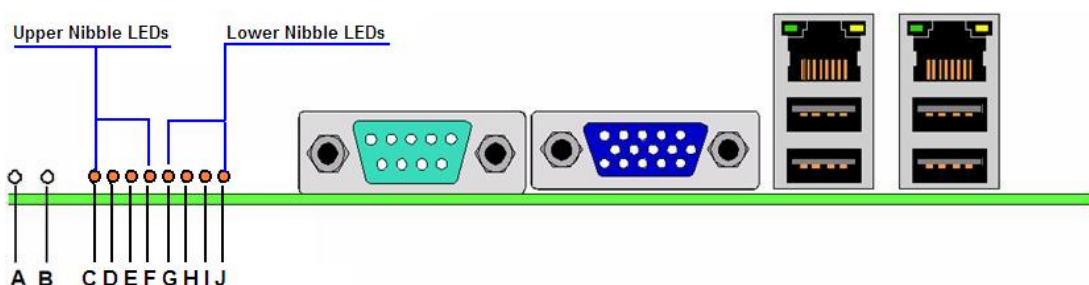
Figure 43. Diagnostic LED Placement Diagram
