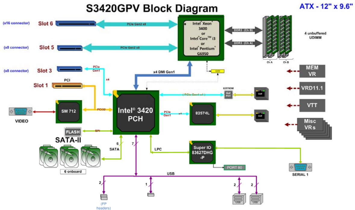
Figure 11. Intel® Server Board S3420GP Functional Block Diagram From S3420GPLC
