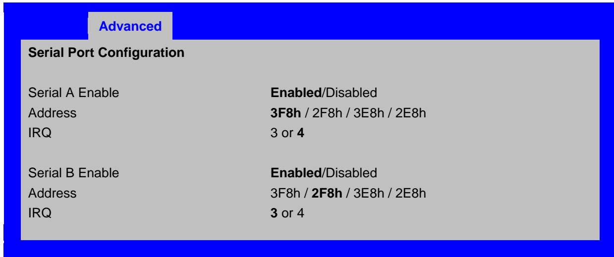
Figure 25. Setup Utility — Serial Port Configuration Screen Display
