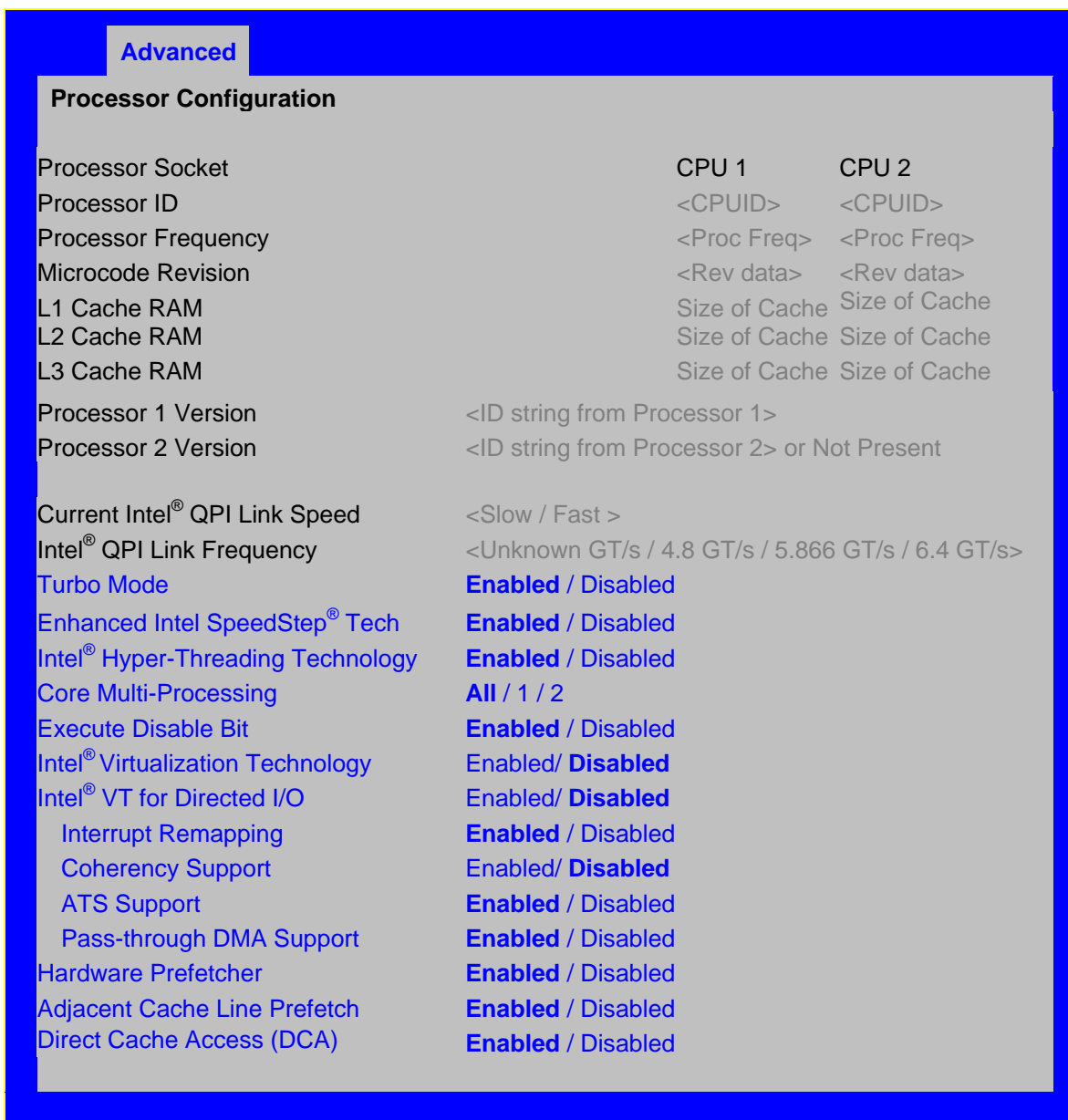
Figure 21. Setup Utility — Processor Configuration Screen Display
