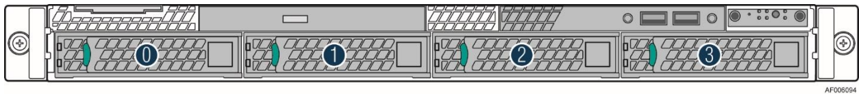
Figure 5. 3.5" Hard Drive Bay - 4 Drive Configuration
