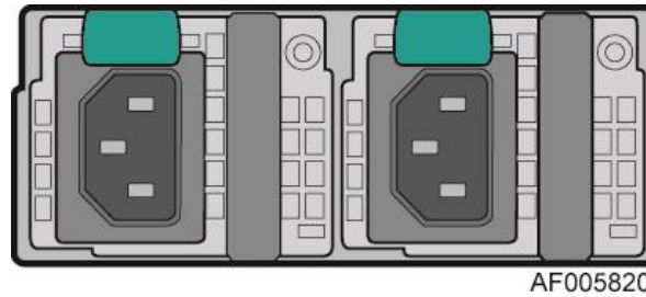
Figure 18. 450W AC Power Supply – Connector View
