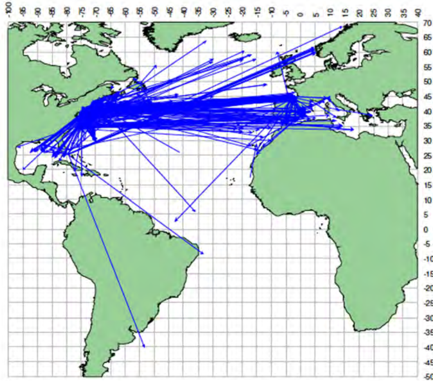
Figure 9.13. Horizontal movements of tagged and recaptured Thunnus thynnus (Bluefin tuna). Direct trajectories between releases and recoveries. Reproduced from ICCAT (2006).
