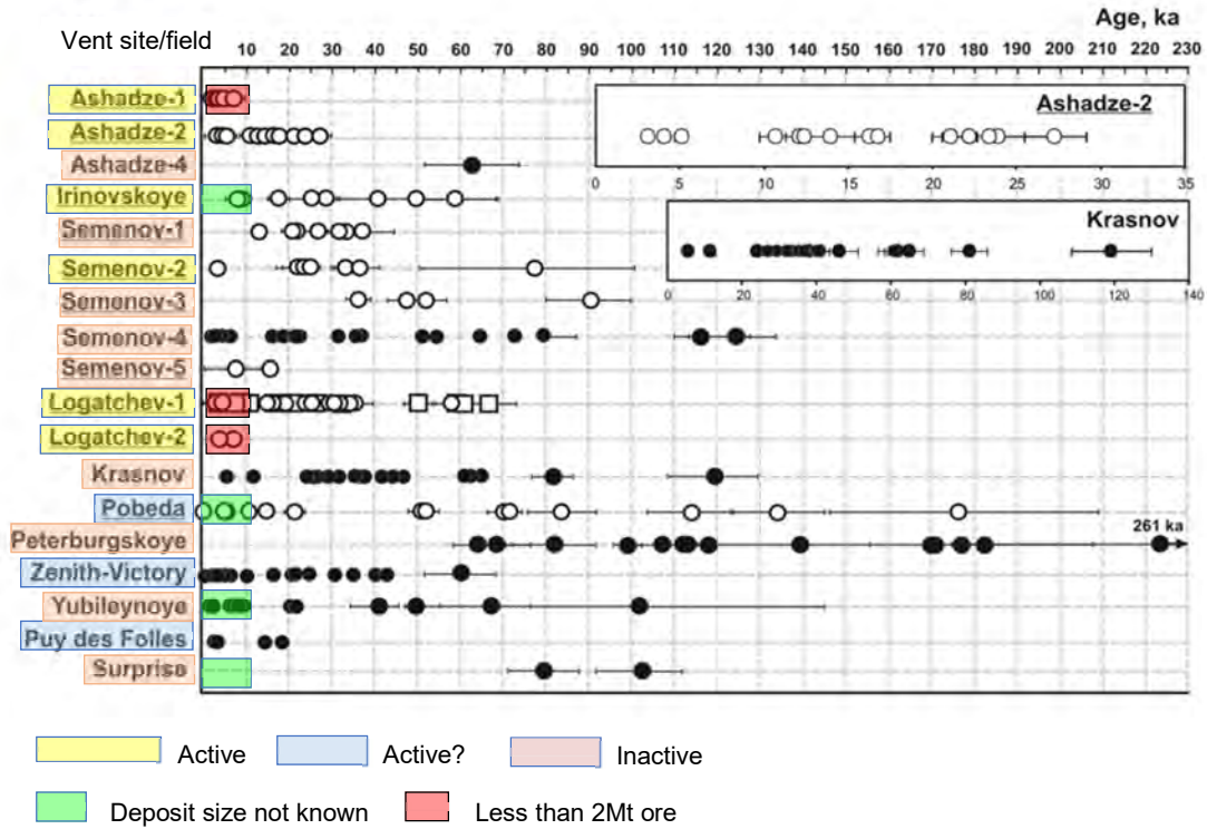
Figure 4.14. Dating results with the 1\sigma variability for SMS deposits at the Russian claim area on the mid-Atlantic Ridge of the North Atlantic. Symbols represent periods of activity. Figure based on data from Cherkashov et al., 2017. (For further explanation see Cherkashov, et al., 2017).
