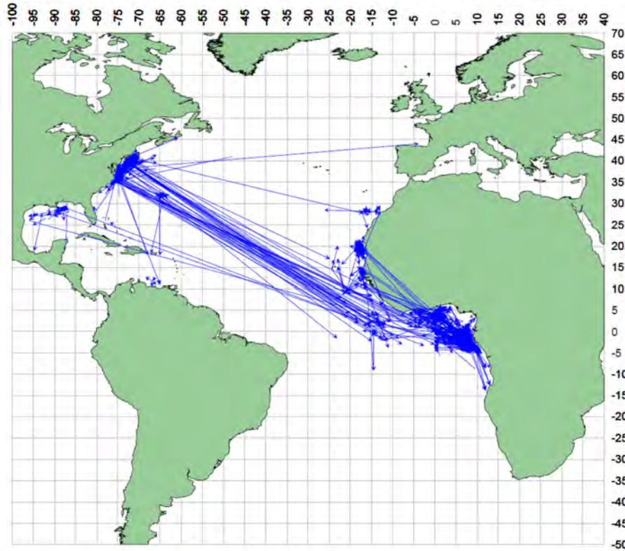
Figure 9.10. Horizontal movements of 1,711 tagged and recaptured Thunnus albacares (yellowfin tuna). Direct trajectories between releases and recoveries. Reproduced from ICCAT (2006).
