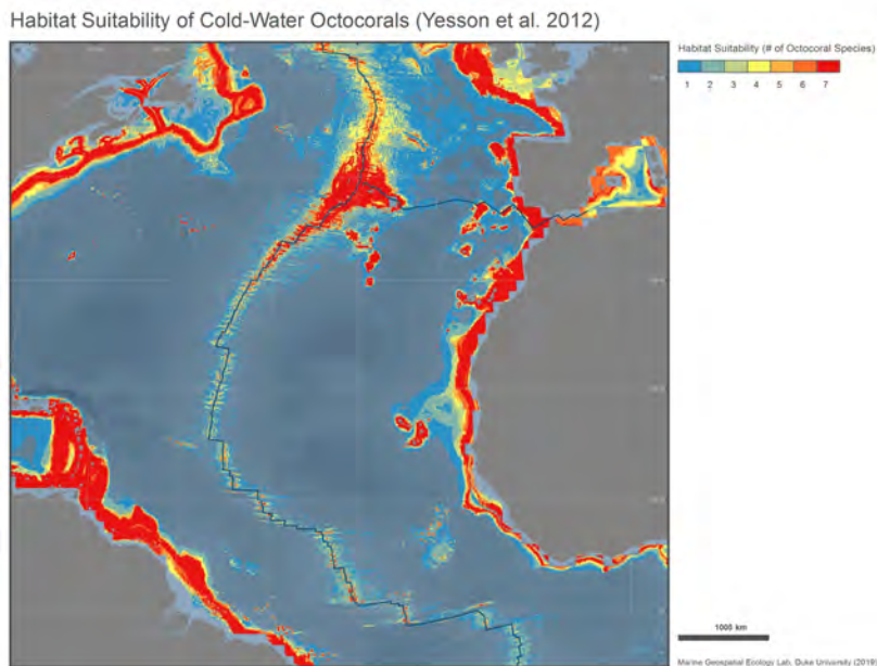
Figure 10.8. Modelled deep-sea octocoral habitat suitability. Map reproduced with permission from Cleary et al., 2019. Data taken from Yesson et al., (2012). Map available: https://ran-s3.s3.amazonaws.com/isa.org/jm/s3fs-public/files/documents/datareport-19nov-lowres.pdf .
