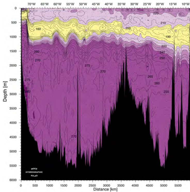
Figure 6.4: West-east sections of (a) potential temperature ( ^{\circ}\text{C} ), (b) practical salinity and (c) oxygen concentration ( \mu\text{mol kg}^{-1} ) across the North Atlantic at 36^{\circ}\text{N} (WOCE line A03), from the WOCE Atlantic Ocean Atlas (Koltermann et al. 2011) based on 1990s data.
