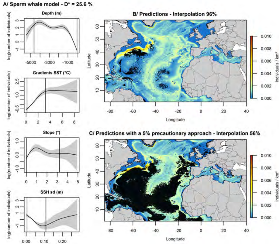
Figure 9.21. Functional relationships for the selected variable (A) and the predicted relative densities of individuals per \text{km}^2 of Physeter macrocephalus (true sperm whales) (B, C). Percentages represent the proportion of the study area defined as interpolation with the gap analysis. Reproduced from Virgili (2018).
