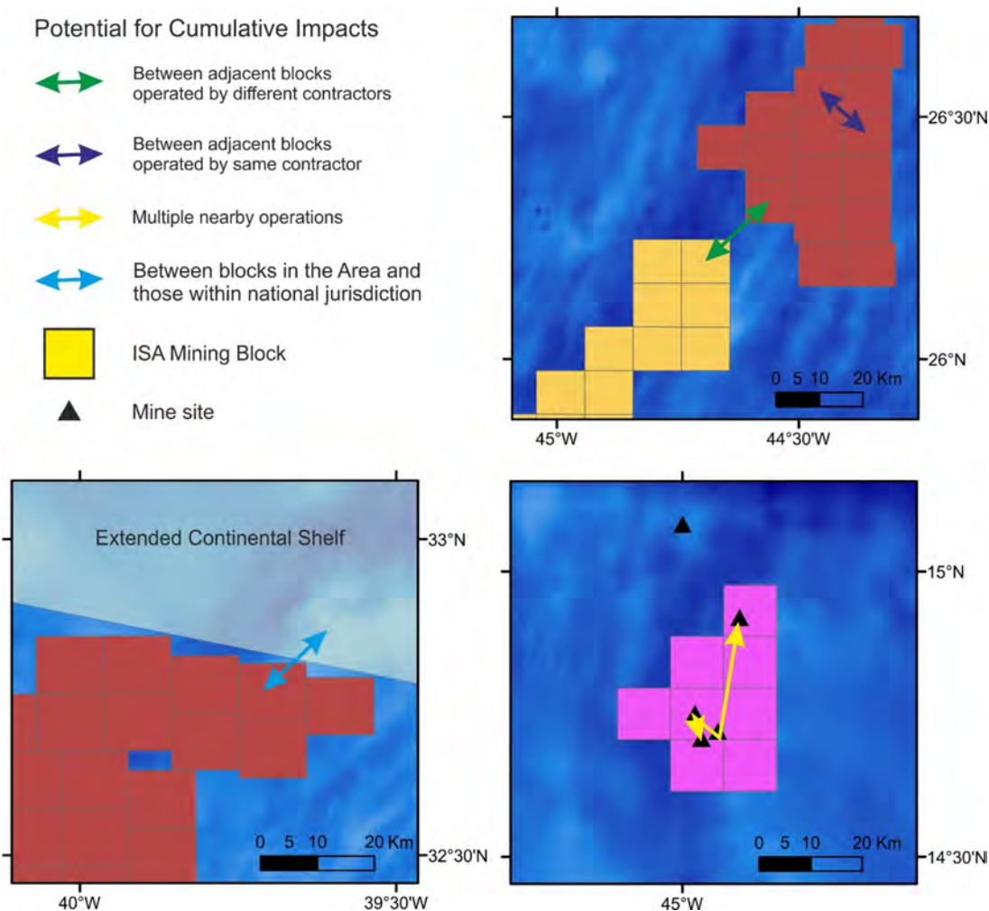
Figure 7.3: Maps showing potential for cumulative impacts. Maps are based on the spatial location of actual ISA exploration blocks (10 x 10 km) and vent sites (as potential mining areas) for scaling. However, the figures do not imply any real mine location information or planned impact scenarios. Blue background represents seabed depth.
