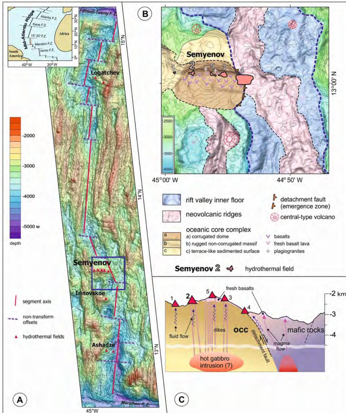
Figure 5.2 The Semenov vent field in the Russian claim area. (A) Shaded-relief bathymetric map of the Mid-Atlantic Ridge between the Fifteen–Twenty Fracture Zone and the Marathon Fracture Zone, showing the location of the hydrothermal fields. The contour interval is 200 m. The box corresponds to the area of Figure B. (B) Morphostructural setting of the Semyenov hydrothermal fields. (C) Interpretative cross-section of the MAR rift valley in the Semyenov cluster (this figure was modified from Pertsev et al., 2012); vertical exaggeration 3:1. Vent site 2 is active whilst all others are inactive. Reproduced from Firstova et al., 2019.
