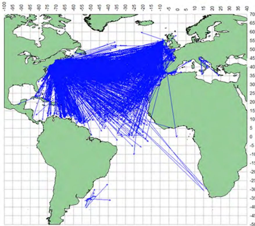
Figure 9.3. Tag and release distribution for Prionace glauca (blue shark) in the Atlantic Ocean, lines describe straight displacement between release and recovery locations. Reproduced from ICCAT (2013).
