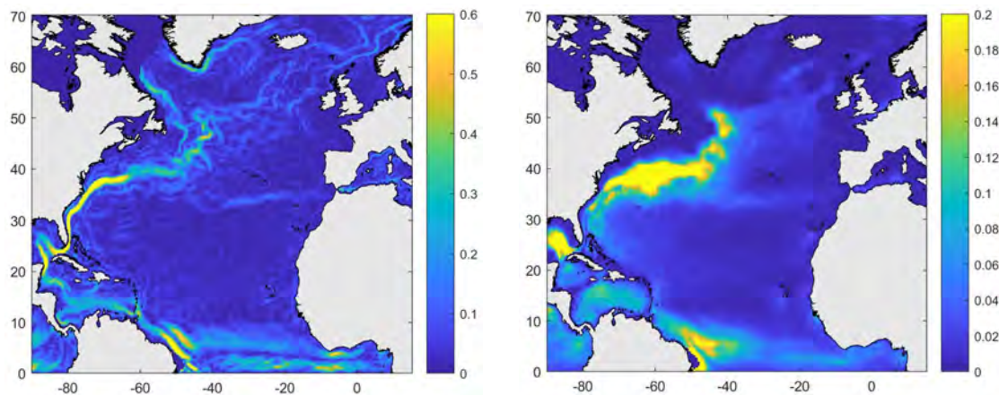
Figure 6.3: (a) Mean surface geostrophic flow speed ( m s^{-1} ), and (b) eddy kinetic energy ( m^2 s^{-2} ) from ten years of satellite altimetry (2009-2018). Values locally exceed the colour scales in high energy areas. (Generated using EU Copernicus Marine Service information, product identifier SEALEVEL_GLO_PHY_L4_REP_OBSERVATIONS_008_047).
