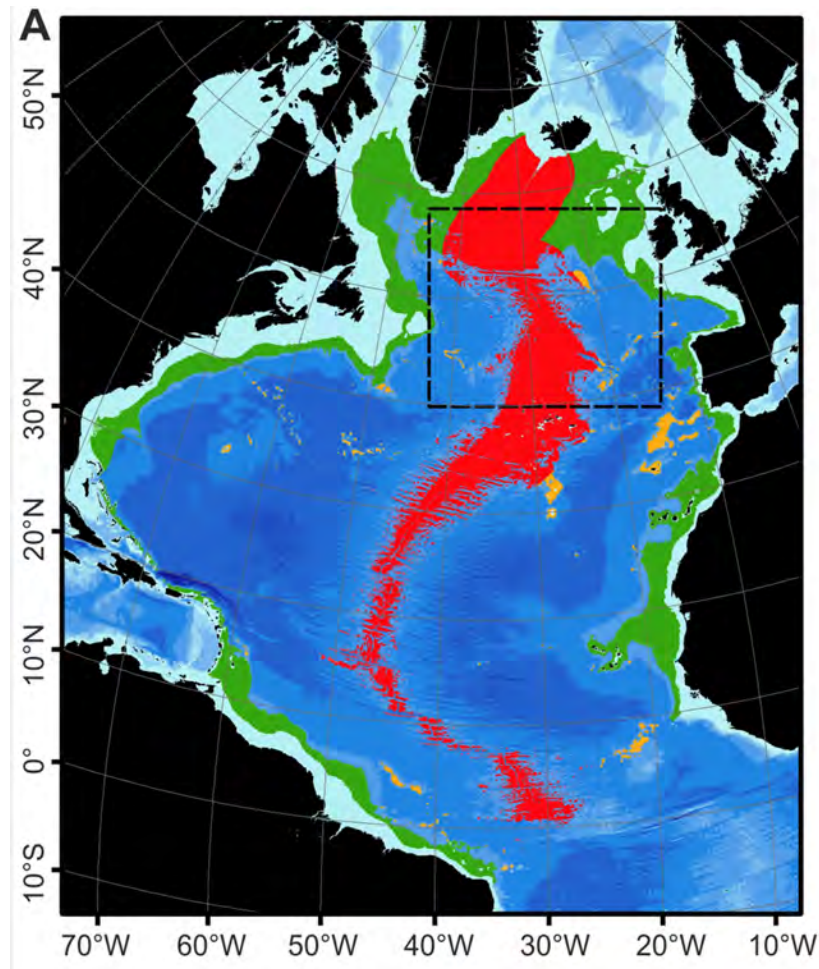
Figure 4.7. The North Atlantic basin showing the lower bathyal zones (depths 800–3500 m) on the MAR (red), continental margins (green) and non-contiguous seamounts (orange). The box represents the ECOMAR study area. Reproduced from Priede et al., (2013).
