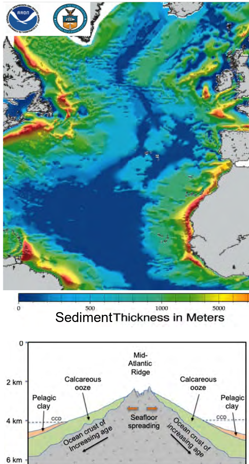
Figure 4.5. A) Upper panel. Sediment thickness in the Atlantic Ocean. From NOAA Total Sediment thickness of the World's oceans and marginal seas https://ngdc.noaa.gov/mgg/sedthick/ B) Lower panel. Cross section of the MAR showing increasing age of crust away from ridge axis and gradual sediment build up away from the ridge axis.
