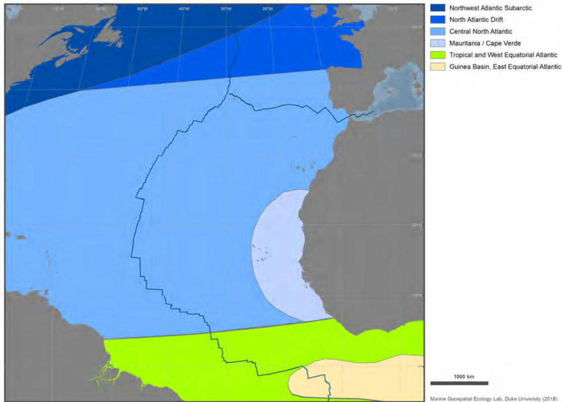
Figure 9.2. Mesopelagic Ecoregions of the North Atlantic Ocean. Map reproduced with permission from Cleary et al., 2019. Data taken from Sutton et al., 2017. Map available: https://rands3.s3.amazonaws.com/isa.org.jm/s3fs-public/files/documents/datareport-19nov-lowres.pdf .
