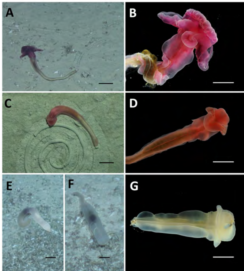
Figure 10.16. Three new species of enteropneustes (free-living acorn worms) discovered on the Mid-Atlantic Ridge (Priede et al. 2012). Yoda purpurata A: On the sea floor before capture. B: Fresh, in chilled aquarium on board ship. Tergivelum cinnabarinum C: On the sea floor before capture, note the spiral trace it produces. D: In aquarium. Allapasus isidis E: curled body floating 0.5 m above the sea floor, F: Settled on the sea floor, G: In aquarium. Scale bars 2 cm long except E, F and G where it is 1 cm long. All specimens were found at around 2500 m depth. Courtesy of Monty Priede and David Shale.
