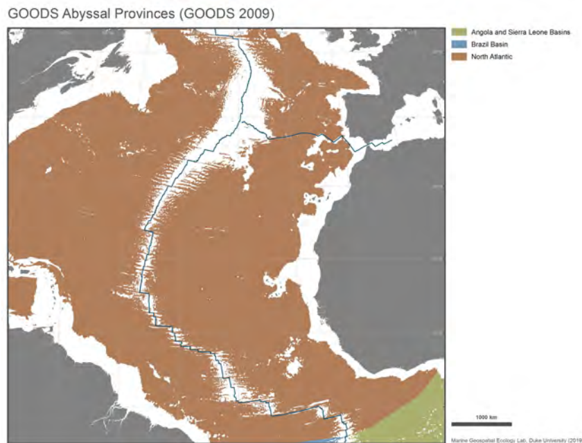
Figure 10.4. GOODS abyssal provinces, depth range 3500 – 6500 m. Map reproduced with permission from Cleary et al., 2019. Data taken from Watling et al., (2013). Map available: https://rands3.s3.amazonaws.com/isa.org/jm/s3fs-public/files/documents/datareport-19nov-lowres.pdf .
