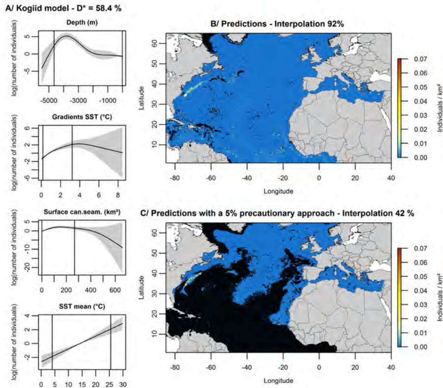
Figure 9.20. Functional relationships for the selected variable (A) and the predicted relative densities of individuals per km 2 of Kogia breviceps (Pygmy sperm whale) and Kogia sima (Dwarf sperm whale) combined (B, C). Percentages represent the proportion of the study area defined as interpolation with the gap analysis. Reproduced from Virgili (2018).
