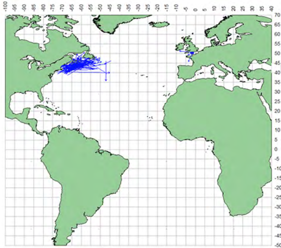
Figure 9.5. Tag and Release distributions Lamna nasus (Porbeagle sharks) in the Atlantic Ocean, lines describe straight displacement between release and recovery locations. Reproduced from ICCAT (2013).
