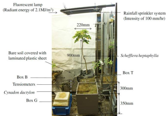
Figure 83. Overview of typical bare, grass and tree test boxes (Ng et al. 2014)
