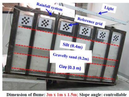
Figure 93. Overview of a typical test for the three-layer landfill cover system using one-dimensional soil column and two-dimensional flume (Ng et al. 2015a; Ng et al. 2015b; Ng et al. 2016a)
