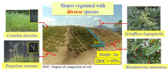
Figure 81. Vegetation in embankment and slopes (Garg et al. 2015; Leung et al. 2015)
