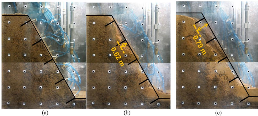
Figure 85. Failure mechanisms of a 60-degree slope reinforced with roots (a) before and after (b) 3 and (5) hours of rainfall in the centrifuge (Ng et al. 2016b; Leung et al. 2017)
