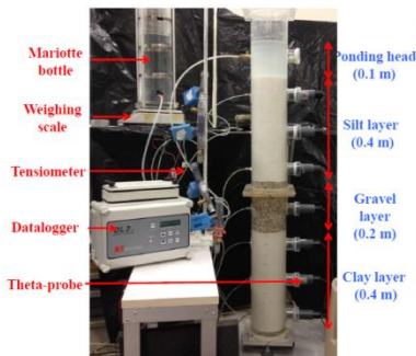
Figure 93. Overview of a typical test for the three-layer landfill cover system using one-dimensional soil column and two-dimensional flume (Ng et al. 2015a; Ng et al. 2015b; Ng et al. 2016a)
