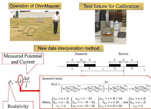
Figure 78. Instrumentation and new data interpretation method using OhmMapper (Niu & Wang 2013; Niu & Wang 2014)
