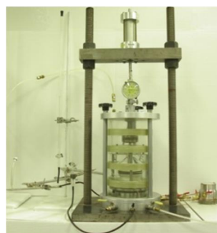
Figure 30. Stress-controlled 3D pressure extractor (Ng et al. 2012)
