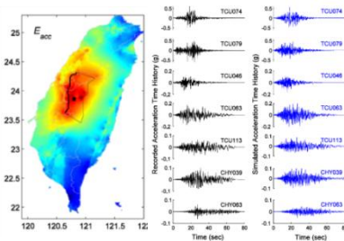
Figure 14. Ground motion simulation, modification using wavelet packets (Huang & Wang 2015)
