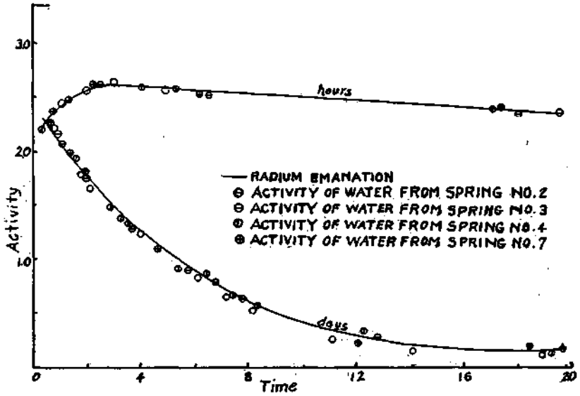
Plate 1. Comparison of decay of activities of waters from Dixon Springs with radium emanation.
