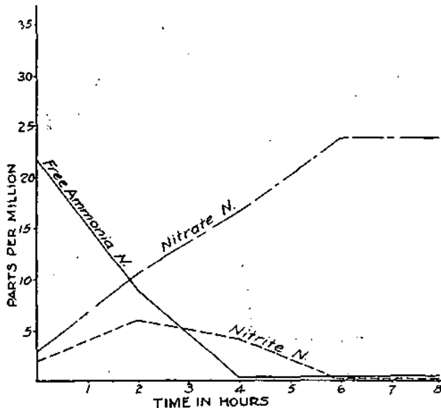
Figure 2.—Aeration of sewage in 3-gallon glass bottles in presence of activated" sludge (1 sludge: 3 sewage). Air distribution through glass tube.
