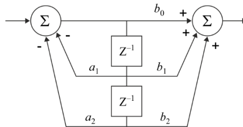
Signal flow diagram as a 2nd order filter
