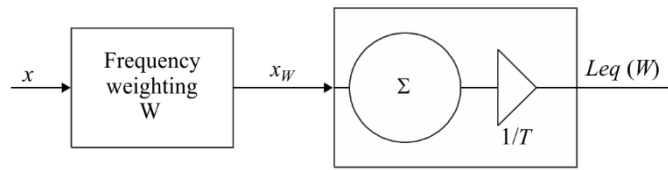
FIGURE 6 Block diagram of the simple energy-based loudness measures
