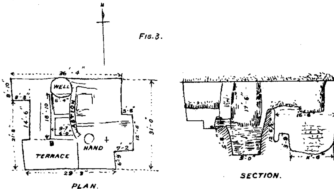
SKETCH PLAN AND SECTION OF EXCAVATION AT KHARĪ KŪĀN.
