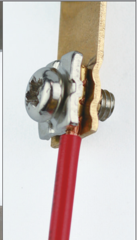
Terminal detail
