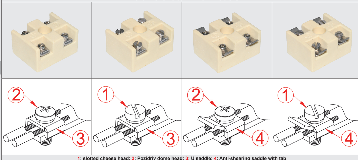
1: slotted cheese head; 2: Pozidriv dome head; 3: U saddle; 4: Anti-shearing saddle with tab
