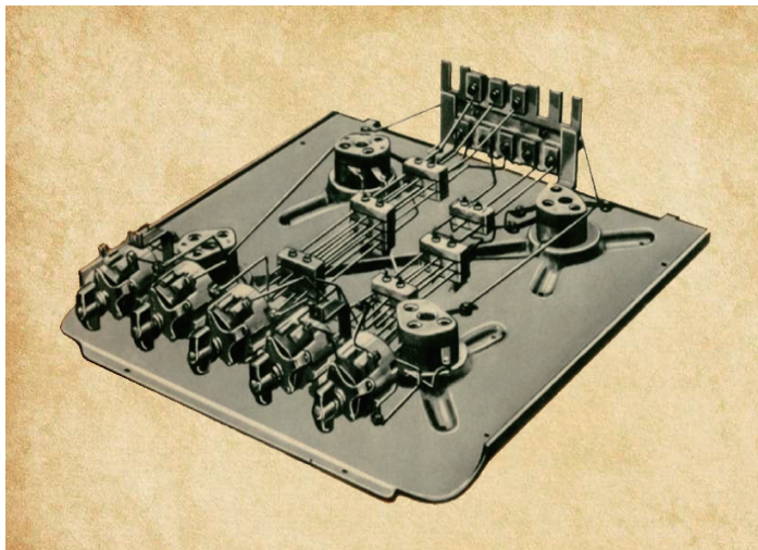
Electrical wiring of the top of an Arthur Martin electric stove (Catalog 1949, Ultimheat Museum). Insulating pieces in steatite and porcelain are omnipresent
