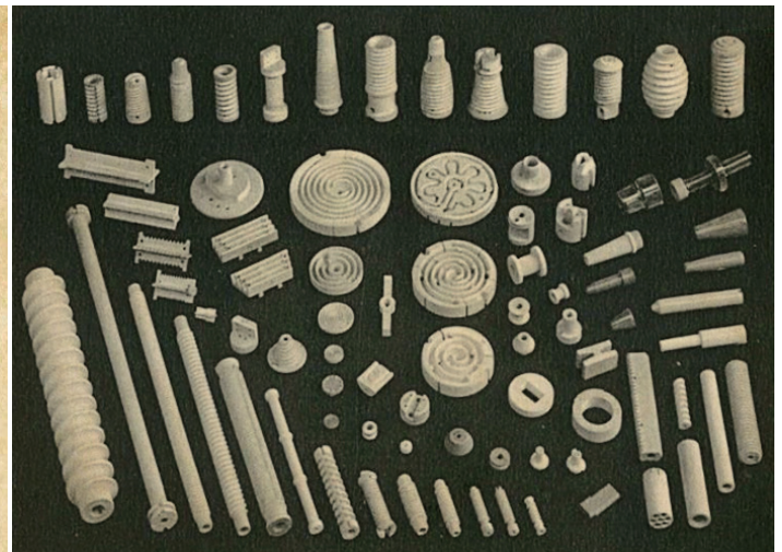
1938 Steatite insulating parts for electrothermal (1938 Catalog La Stéatite industrielle, Ultimheat Museum)
