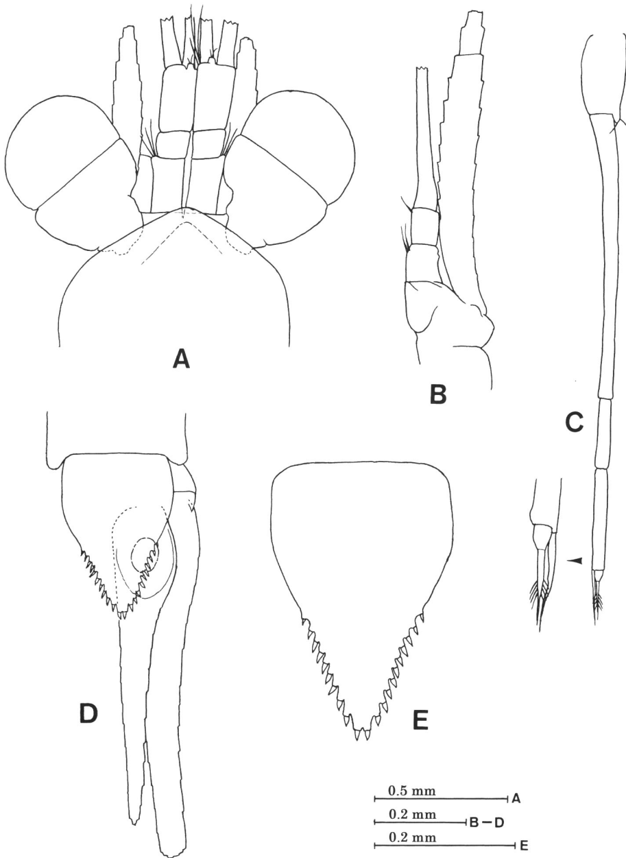
Fig. 8. Anisomysis (Anisomysis) australis Zimmer, 1918, A, B, E: gravid female (5.1 mm); C, D: male (4.4 mm). A, anterior part of body; B, antenna; C, fourth pleopod; D, uropod and telson; E, telson.
