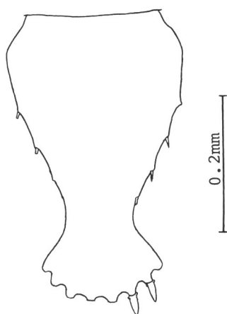
Fig. 1. Anisomysis ( Pseudanisomysis ) hispida Pillai, 1973. Telson.
