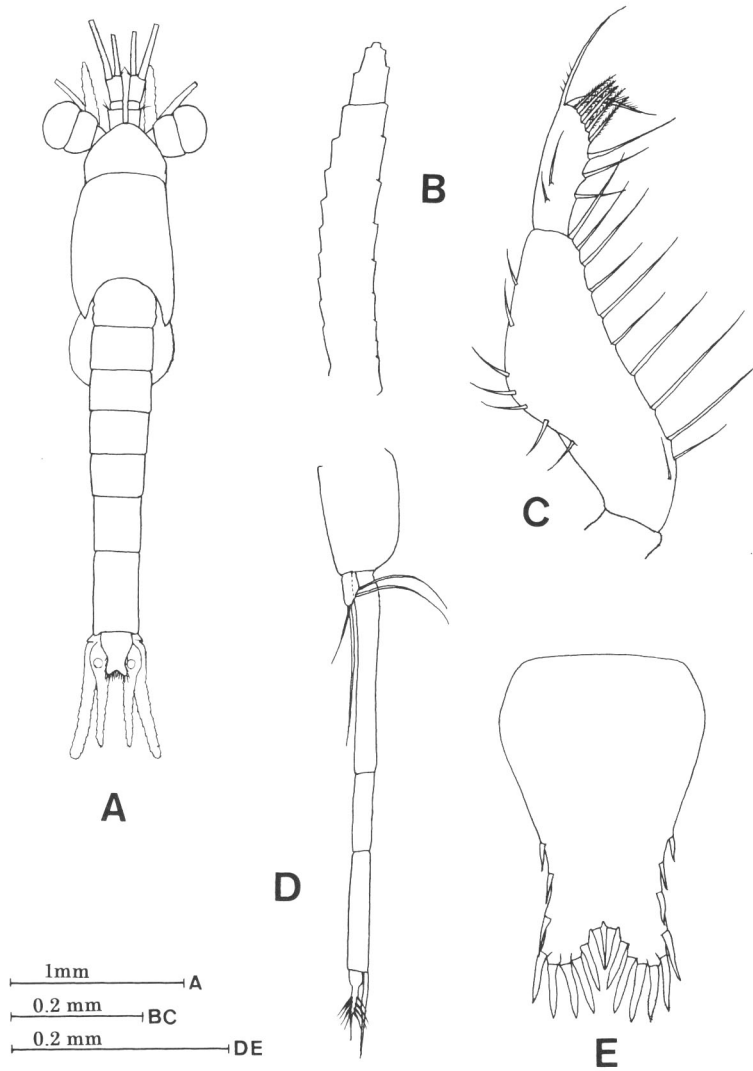
Fig. 9. Anisomysis (Anisomysis) aikawai Ii, 1964, from Nomo. A–C, E: adult female; D: adult male. A, adult female in dorsal view; B, antennal scale; C, mandibular palp; D, fourth pleopod of male; E, telson.
