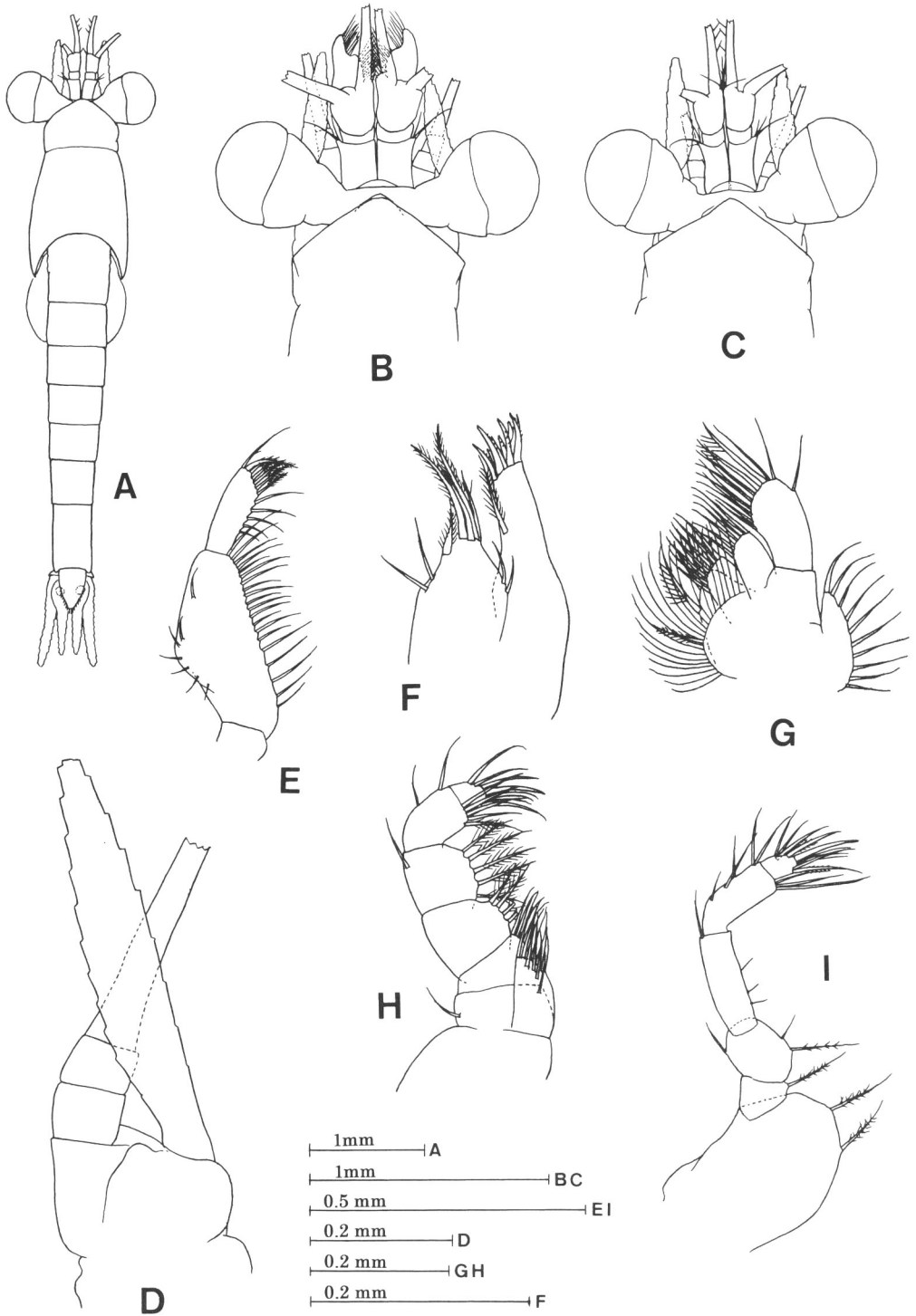
Fig. 6. Anisomysis (Anisomysis) mixta Nakazawa, 1910, from Nomo, A, C, F–I: adult female; B, D, E: adult male. A, whole body in dorsal view; B, anterior part of body; C, anterior part of body; D, antenna; E, mandibular palp; F, maxillule; G, maxilla; H, endopod of first thoracic limb; I, endopod of second thoracic limb.
