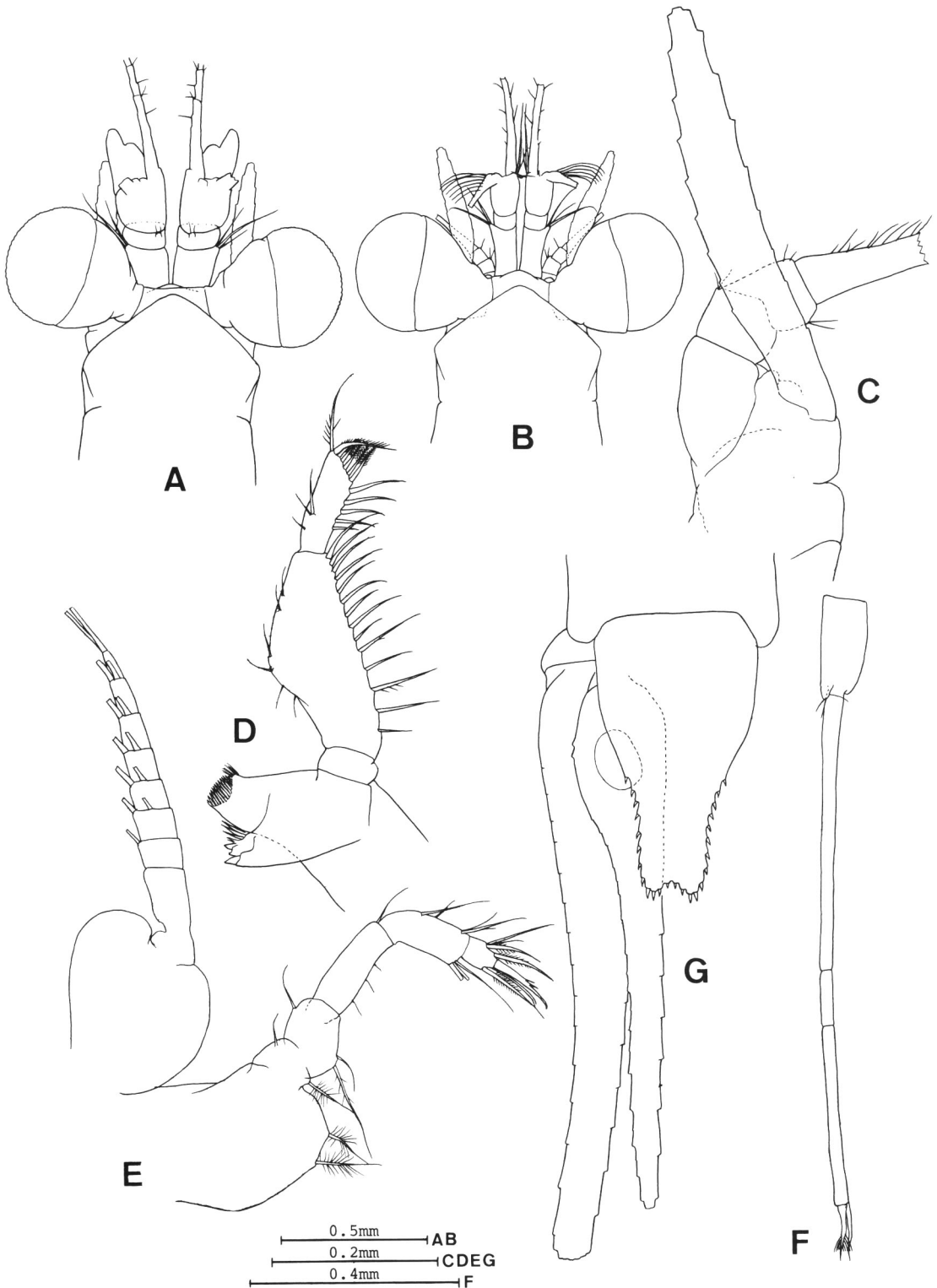
Fig. 14. Anisomysis (Anisomysis) parvispina n. sp., A, F, G, holotype; B, allotype; C–E, one of female paratypes (3.3 mm). A, anterior part of body; B, anterior part of body; C, antenna; D, mandible and mandibular palp; E, second thoracic limb; F, fourth pleopod of male; G, uropod and telson.
