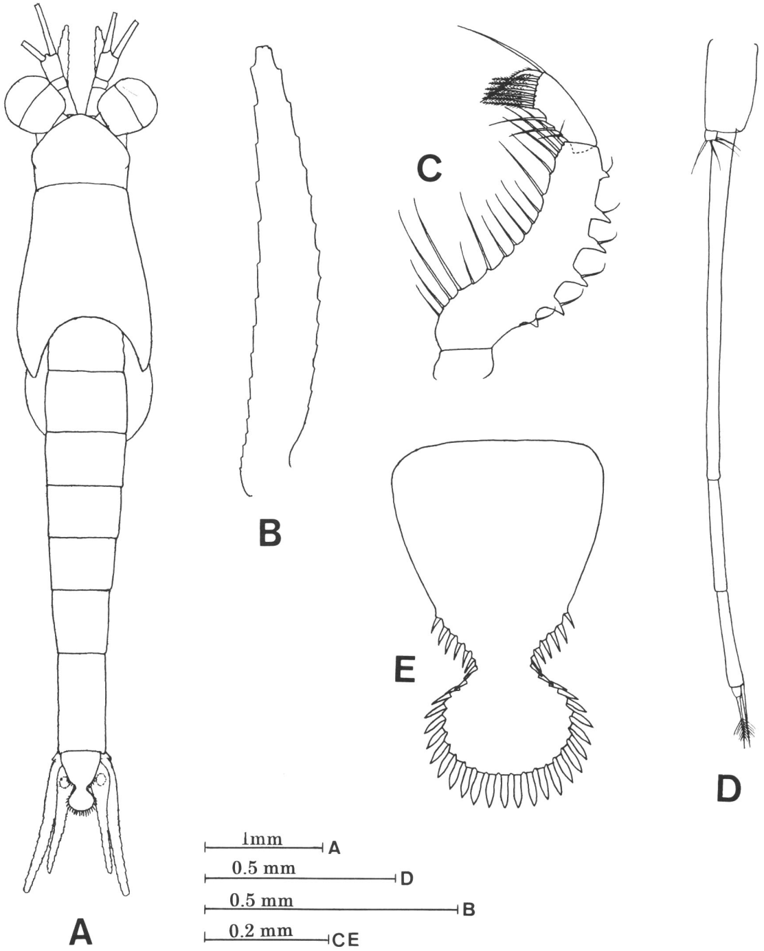
Fig. 2. Anisomysis (Paranisomysis) ijimai Nakazawa, 1910, from Heda, A–C, E: adult female; D: adult male. A, whole body in dorsal view; B, antennal scale; C, mandibular palp; D, fourth pleopod; E, telson.
