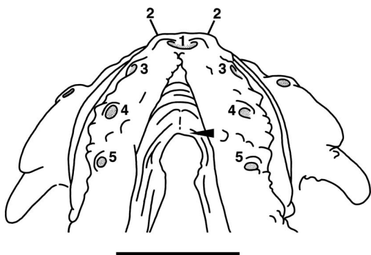
Fig. 2. Ventral view of head of Cocotropus izuensis sp. nov., KPM-NI 22797, holotype, 40.2 mm SL, east coast of Izu Peninsula, Japan. Arrow head and numbers indicate anterior tip of isthmus and sensory openings of lower jaw, respectively. Most papillae underlain by a tiny buried scale are not shown. Scale indicates 3 mm.
