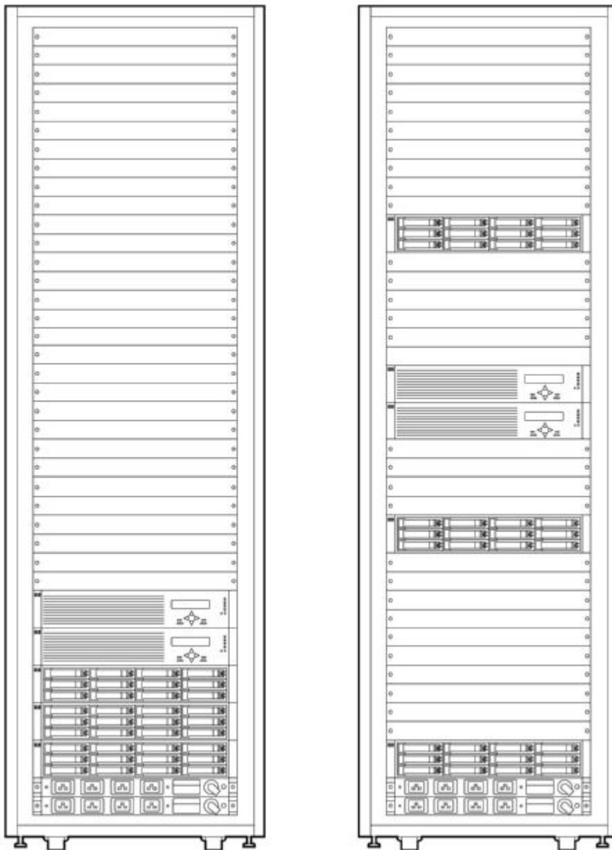
Multiple Product Racking Configuration
