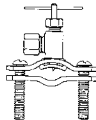
104SCSD Self Drilling Valve Assembly fits 3/8" thru 1-3/8" O.D. Copper Tubing
