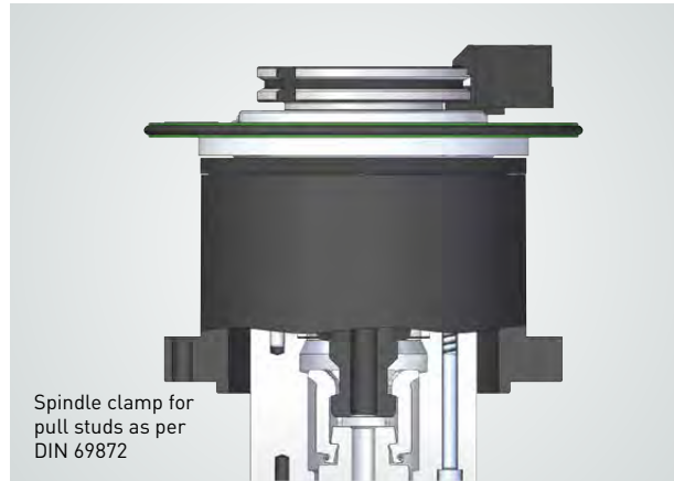
Tool clamping
