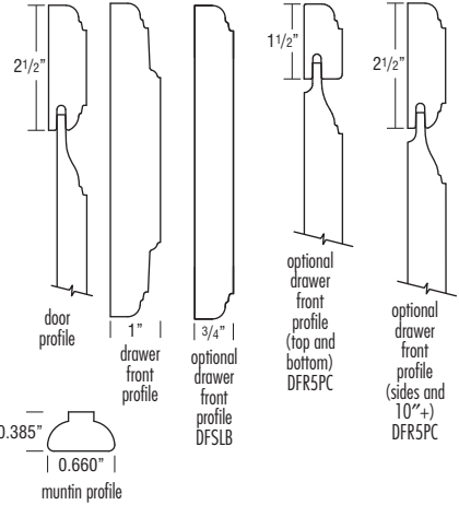
Optional Drawer Front: Raised 5-Piece (DFR5PC)
