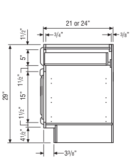
DESK BASE CABINET
