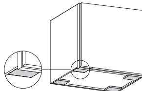
PREPARE CABINET FOR FINISHED BOTTOM (PFINBTMB)
