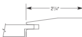
Drawer Rail/Center Panel Detail
