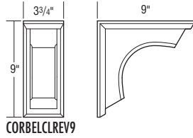
9" CLASSIC REVIVAL CORBEL R•24
