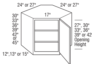
DW302424 L or R - DW452727 L or R
