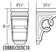
10" CELTIC CORBEL R•24
