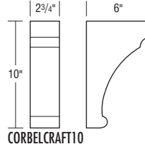
10" CRAFTSMAN CORBEL R•23
