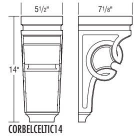
14" CELTIC CORBEL R•25
