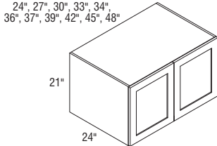
W242124-W372124 Butt doors W392124-W482124CS Center mullion
