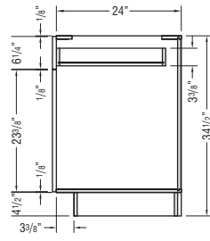
BASE CABINET
