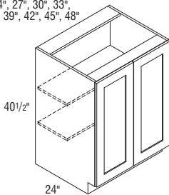
B2440FH-B3640FH Butt doors B3940FH-B4840FHCS Center mullion
