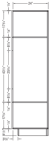
SINGLE OVEN CABINET
