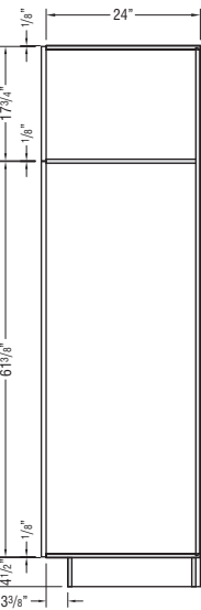
PANTRY CABINET
