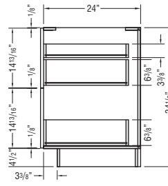
TWO-DRAWER BASE CABINET with ROLL TRAY
