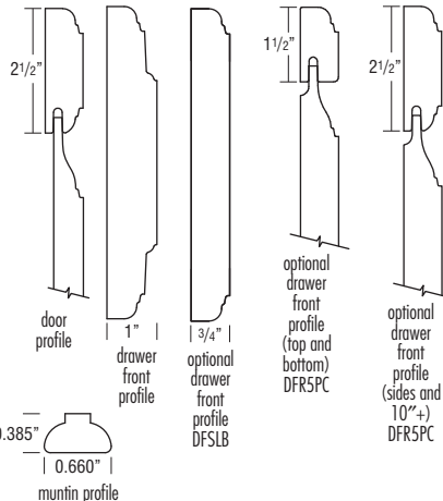
Optional Drawer Front: Raised 5-Piece (DFR5PC)
