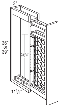
WBCPOKCUP336 WBCPOKCUP339
