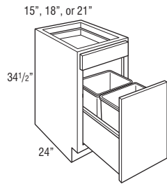
BWB152 BWB18 BWB21
