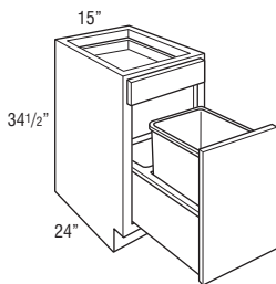
BWB15
