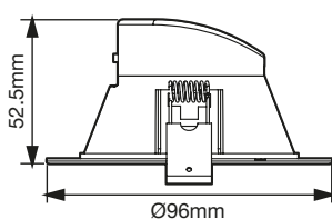
Cut out: 72mm Ø96mmx52.5mm
