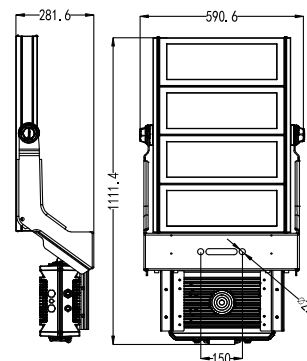
1200W 590.6x281.6x1111.4mm
