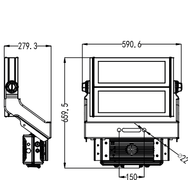
600W 590.6x659.5x279.3mm
