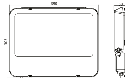
120/160/200W 390x305x58mm
