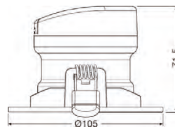
10W Cut out: 92mm Ø105x71.5mm
