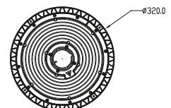
200W Ø320x121.3mm
