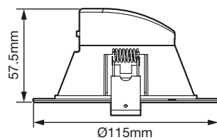
Cut out: 90mm Ø115mmx57.5mm
