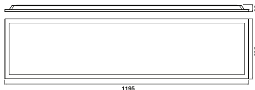
36/30W 295x1195x32mm
