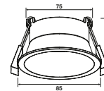
Deep Recess LDVDLMODADR80 Cut out: 75-80mm
