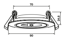
Adjustable LDVDLMODAG80 Cut out: 75-80mm
