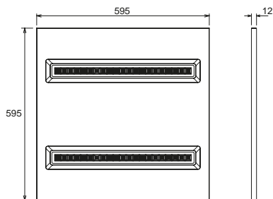
33W 595x595x12mm
