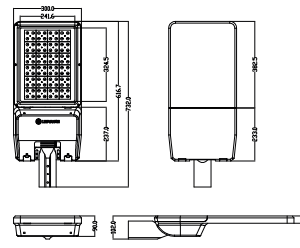
179W, 210W 732x300x102mm
