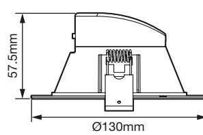
Cut out: 110mm Ø130mmx57.5mm
