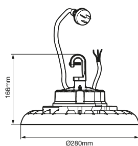
60W/80W/100W Ø280x166mm
