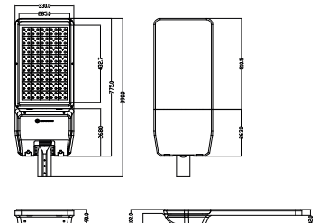
256W, 300W, 320W 890x330x102mm
