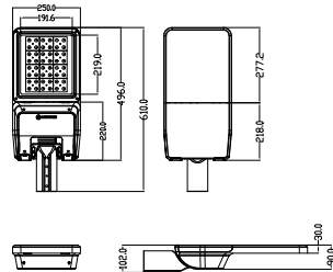
90W, 120W 610x250x102mm
