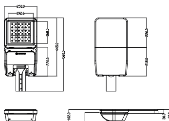
21W, 42W, 72W 560x250x102mm
