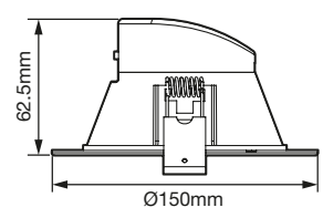
Cut out: 125mm Ø150mmx62.5mm
