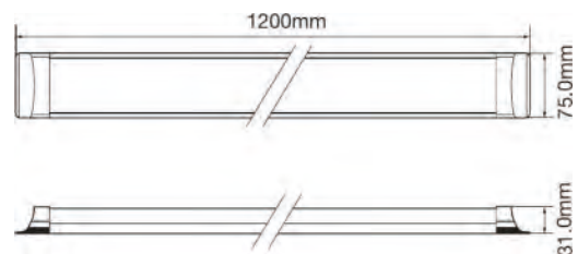
40W 1200x75Mx30.5mm
