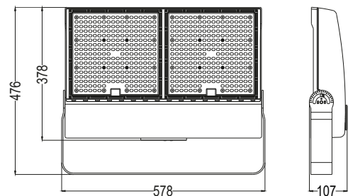
330/400/500W 578x456x100mm
