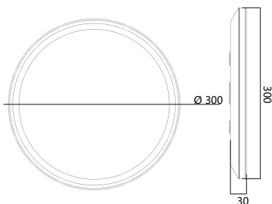
18W Ø300x30mm
