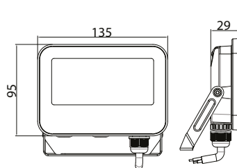
6/8/10W 135x95x29mm
