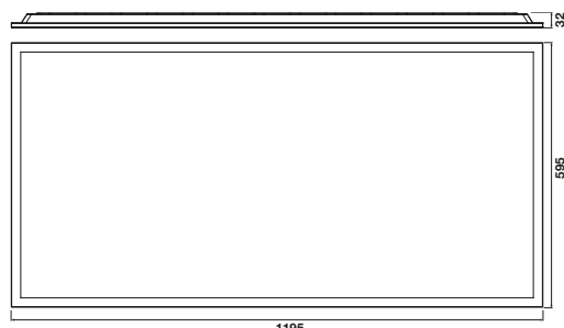
60/50W 595x1195x32mm
