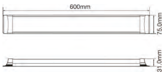
20W 600x75x30.5mm
