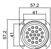
LKS 19 19 pins size 12
