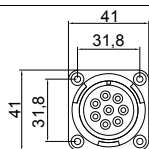
LK 08 Size 22 - 8 pins size 12
