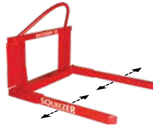
SQ-80 SQUEEZER™ 54" hydraulic arms grab bales and squeeze securely for transport. Tilts the bale from end to side, opens to 78", closes to 48" and includes cylinders and hoses.
