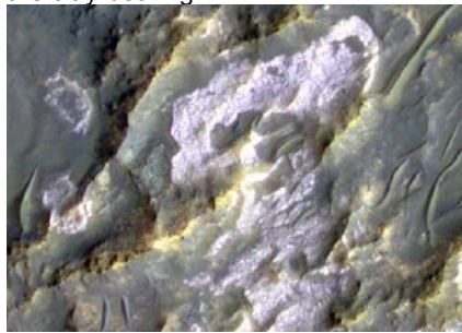
Fig. 4. HiRISE image of the polygonally fractured surface of glowing terrain. Thermal IR properties are consistent with a high chloride content (type location, Terra Sirenum).
