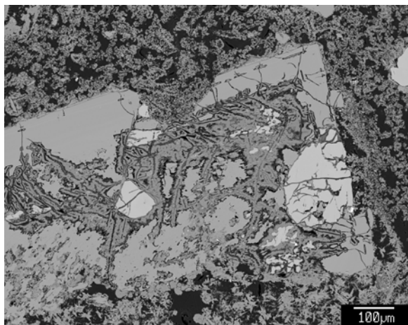
Figure 2a. BSE image of partially altered plagioclase (light gray) in which the calcic core has been replaced by amorphous SiO 2 (dark gray).
