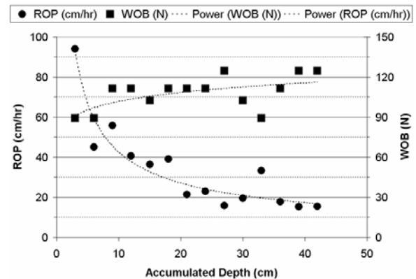
Figure 2. Rate of Penetration (ROP) and Wight on Bit (WOB) vs. Accumulated Depth for a single bit in 100 MPa Keweenaw Basalt. [2]
