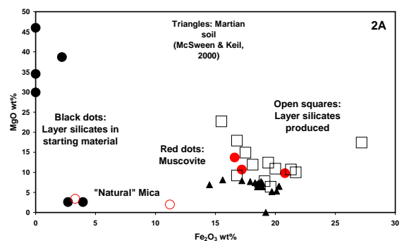
Figure 2A: Fe 2 O 3 vs. MgO (wt%) in KOSI starting material (black dots) and modified layer silicates (open squares). KOSI-2 muscovite (solid red dots) is presumably Fe-enriched muscovite from the starting material by comparison with “natural” mica compositions (open red circles). Martian soil compositions [5] are for reference only (solid triangles).
