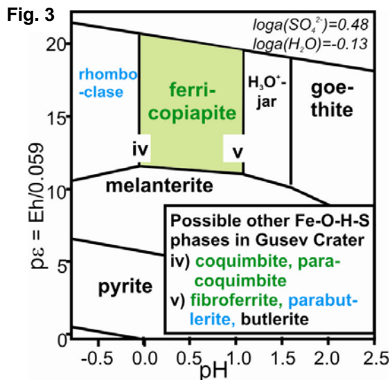
Figure 1: \text{Fe}_2\text{O}_3\text{-H}_2\text{O-SO}_3 diagram [modified after 11] showing the stability of different \text{Fe}^{3+} -sulfates, goethite and solution.
