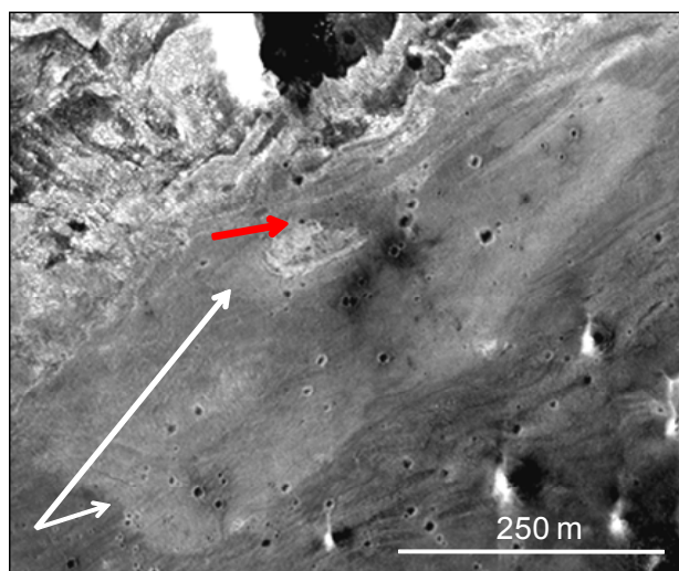
Fig. 2. East mound: inner and outer tonal anomalies (white arrows) and terraced side with apical depression (red arrow). HiRISE image PSP_002812_1855.
