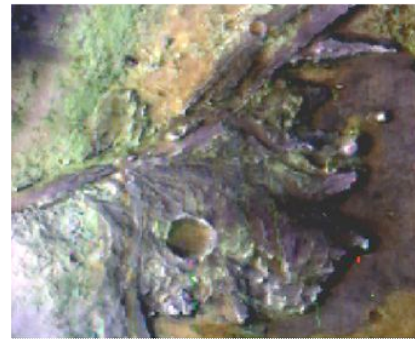
Fig. 3. CRISM IR false color image of an intra-crater fan. Green material in the base of the fan is phyllosilicate-bearing (type location, Jezero crater).
