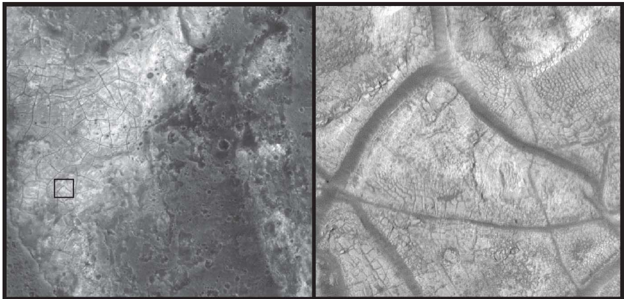
Figure 1: MOC image M1800673 (at left) showing the “polygons” sub-unit of the light-toned, clay-bearing unit in the Mawrth Vallis region. OMEGA detects nontronite and ferrihydrite in this deposit [7]. The MOC image is 3 km across. The inset shows the location of HiRISE image PSP_001454_2030 (at right), which reveals the morphology of two scales of fractures present in this unit. The question remains open as to whether the cracks are related to desiccation of smectites in these rocks.
