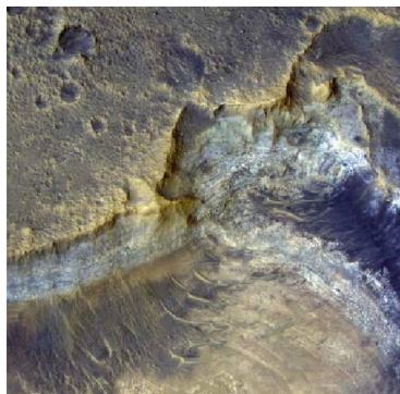
Fig. 1. HiRISE image of Noachian layered clays (type location, Mawrth Vallis). The light-colored materials are clay-bearing.
