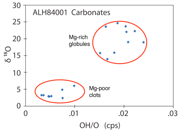
Fig. 3. Ion microprobe analysis of \delta^{18}\text{O} VSMOW vs. count rate on OH normalized to oxygen for carbonates in ALH84001. Carbonate globules ( \delta^{18}\text{O} > 13 ) contain significantly more OH than clots ( \delta^{18}\text{O} < 6 ).
