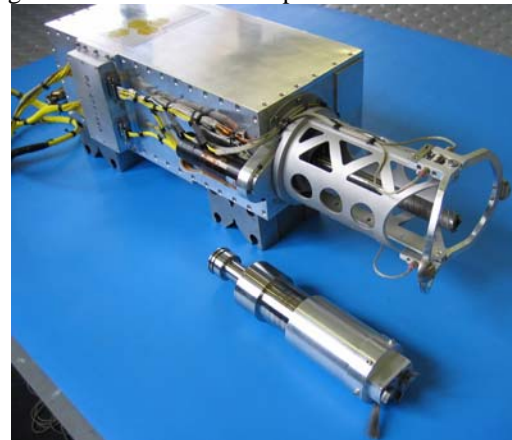
Figure 3. Corer Abrade Tool (CAT) can acquire rock cores and abrade rocks. It weighs less than 4 kg and is designed to be arm mounted.
