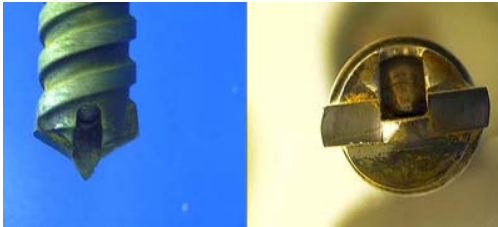
Figure 4: Detail of Sampling Tip (Door Closed) of the Sample Acquisition and Transfer Mechanism (SATM) drill.
