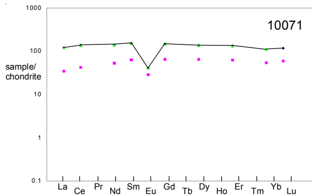
Figure 6: Normalized rare-earth-element composition for high-K basalt 10071 (the line) compared with that of low-K basalt 10020 and high-K basalt 10049 (the dots) (data from Wiesmann et al. 1975).
