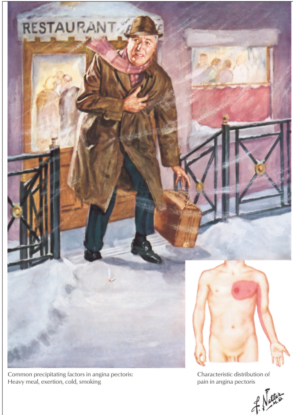
Figure 3. Angina Pectoris
