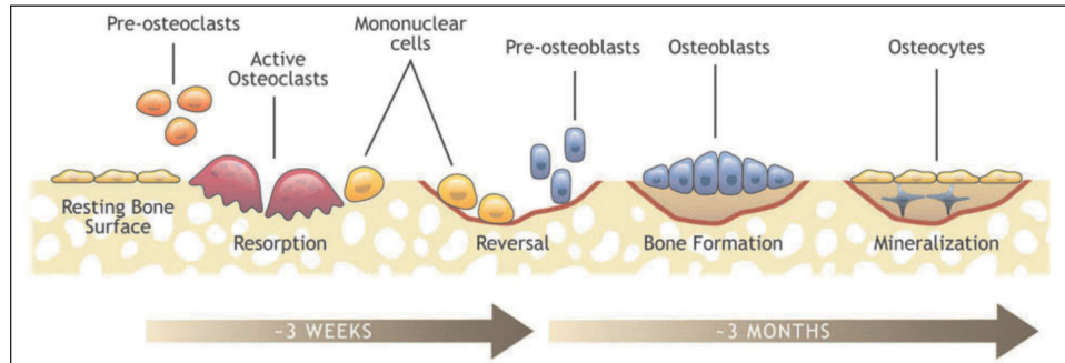
Figure 1. Bone Remodeling
