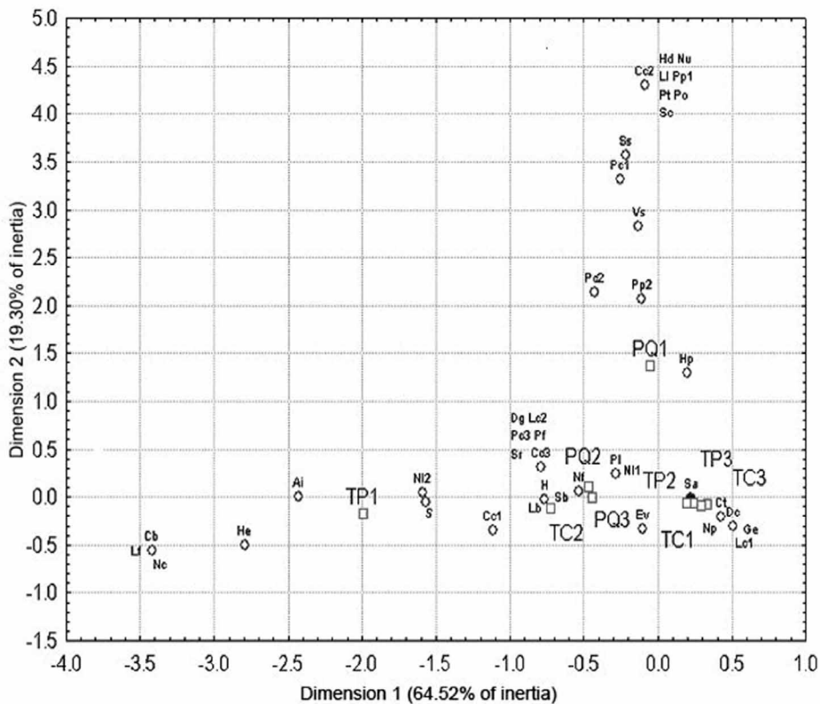
FIGURE 4. Correspondence analysis ordination plot: Dimension 1 is related to abundance of S. alveolata (from left to right), Dimension 2 is related to the turbidity tolerance gradient (bottom to top). Species legend: Ai = Arabella iricolor , Cb = Caulleriella bioculata , Cc1 = Caulleriella cf. alata , Cc2 = Ceratonereis costae , Ct = Cirriiformia tentaculata , Cc3 = Clymenura clypeata , Dc = Dasybranchus caducus , Dg = Dasybranchus gajolae , Ev = Eulalia viridis , Ge = Goniada emerita , Hd = Hediste diversicolor , He = Hydroides elegans , Hp = Hydroides pseudouncinatus , Lc1 = Lanice conchylega , Lc2 = Lepidonotus clava , Lf = Scoletoma funchalensis , Lg = Lumbrineris gracilis , Ll = Lumbrineris latreilli , N11 = Nainereis laevigata , Nc = Neanthes caudate , Nu = Nematonereis unicornis , Nf = Nereis falsa , Np = Nereis pelagica , N12 = Notomastus lineatus , Pc1 = Perinereis cultrifera , Pd = Platynereis dumerilii , Pp2 = Polyophthalmus pictus , Pl = Pomatoceros lamarcki , Pt = Pomatoceros triqueter , Pc2 = Pontogenia chrysocoma , Pc3 = Minuspio cf. cirrifera , Po = Protoaricia oerstedii , Pf = Pseudoleiocapitella fauveli , Sa = Sabellaria alveolata , S = Sabellaria spinulosa , Sr = Dorvillea (Schistomeringos) rudolphii , Sc = Serpula concharum , Sb = Sthenelais boa , S = Syllidae, Vs = Vermiliopsis striaticeps .
