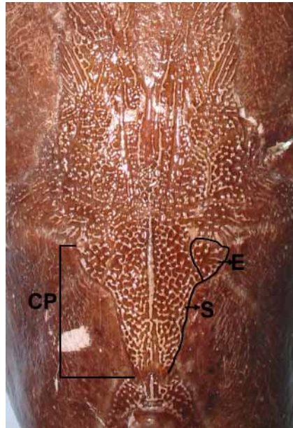
FIGURE 6. Head shield of a female specimen (STRI 5715, 16 mm supraoccipital process length) of Notarius insculptus . CP: complex process; E: epioccipital (= epiotic); S: supraoccipital.
