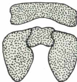
FIGURE 3. Palatine teeth patches of Notarius biffi (after Kailola and Bussing, 1995).
