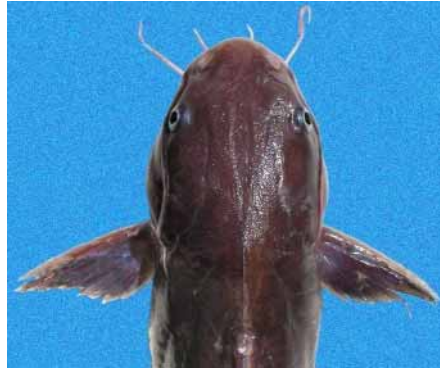
FIGURE 5. Dorsal view of head of a female specimen (STRI 5715, 60 mm HL) of Notarius insculptus , from the Pacific coast of Panamá (photo by D.R. Robertson).
