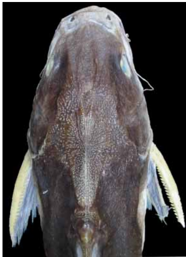
FIGURE 2. Dorsal view of head of a female paratype (UCR 2451-2, voucher 95-7; 72 mm HL) of Notarius biffi , from the Pacific coast of Costa Rica.
