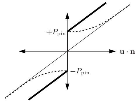
FIG. 6. A more realistic relationship between the resistive pressure at the interface and the normal velocity. Here, [\lambda + D_{\text{visc}} \mathbf{u} \cdot \mathbf{n}] is plotted as the thick line. Note how the interface pressure increases with increasing velocity. The dashed line depicts a slightly more nonlinear relationship [\lambda + D_{\text{visc}} \mathbf{u} \cdot \mathbf{n} + G_{\text{fric}}(\mathbf{u} \cdot \mathbf{n})] [see Eq. (16)]. The qualitative form of the dashed line has been shown in the work of Refs. 54–57. Note: the dashed line asymptotes toward the thin line D_{\text{visc}} \mathbf{u} \cdot \mathbf{n} .
