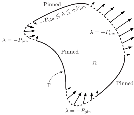
FIG. 5. A two dimensional droplet (top view) with parts of the boundary pinned (electrode grid not shown). The pinned regions are denoted by a solid line; unpinned regions are shown as a dashed line with velocity arrows indicating direction of motion. An outward motion is considered positive ( \mathbf{u} \cdot \mathbf{n} > 0 ) and an inward motion is negative ( \mathbf{u} \cdot \mathbf{n} < 0 ). The pinning variable \lambda is defined on the boundary \Gamma of the droplet. On the unpinned regions, the value of \lambda saturates to \pm P_{\text{pin}} . On the pinned regions ( \mathbf{u} \cdot \mathbf{n} = 0 ), \lambda varies between -P_{\text{pin}} and +P_{\text{pin}} (see Fig. 6). In our simulations, |\lambda| < P_{\text{pin}} is used to indicate where the boundary is pinned.
