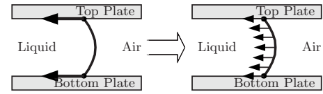
FIG. 4. Contact line force averaging (cross-sectional slice of EWOD device shown; z -axis is in the vertical direction). Contact line friction is a force that is active along the three-phase contact line. On the left, the contact line pinning force is shown concentrated at the contact line (at both the floor and ceiling). On the right, the pinning force has been redistributed over the channel height. Since the governing EWOD fluid equations have been averaged along the channel height, we average the contact line pinning force across the channel height also. This redistributes the force from a length of contact line (at floor and ceiling) to a vertical strip along the liquid-gas interface. This allows the line pinning force to be included in the pressure boundary conditions as an additional pressure term [see Eq. (13)].
