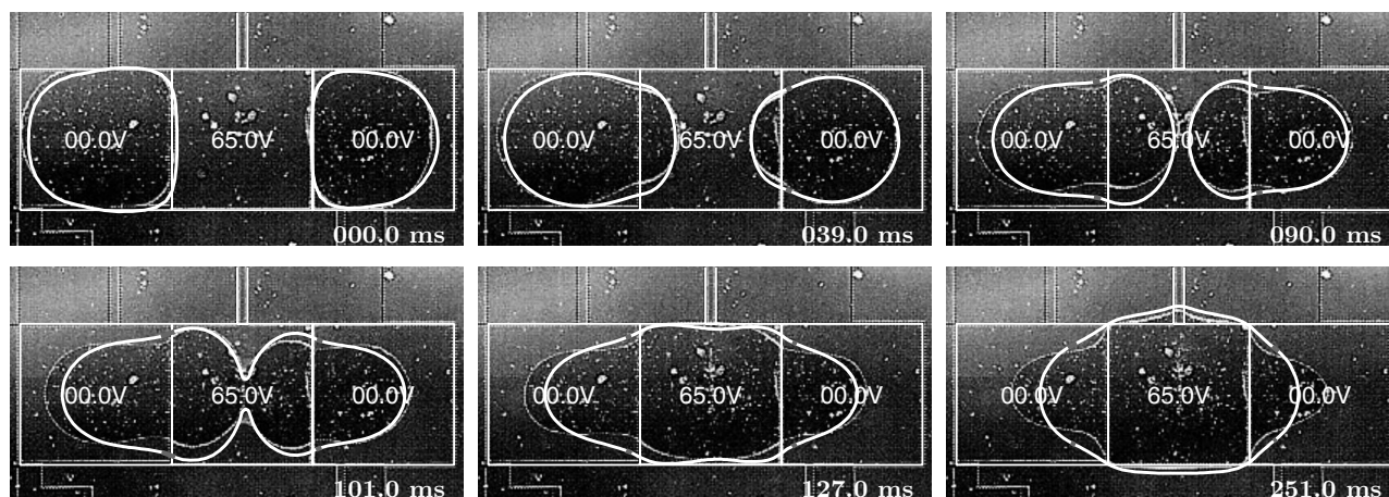
FIG. 12. Joining water droplets experimental results with simulation overlay (solid curve is the simulation). Frames show video snapshots of the experiment (experimental data courtesy of C. J. Kim and Jian Gong at UCLA). The applied voltage (65 V on the center electrode only) causes the two side droplets to flow together and eventually merge. Each electrode is approximately square with a side length of 1.5 mm. The simulation matches the experiment fairly well in the first four frames. However, the pinning behavior in the experiment is significantly different than the simulation in the last two frames. We believe that the sharp snap together of the droplets during coalescence makes this case more sensitive to modeling uncertainties than the move or split cases (enhanced online). [URL: http://dx.doi.org/10.1063/1.3254022.3 ]
