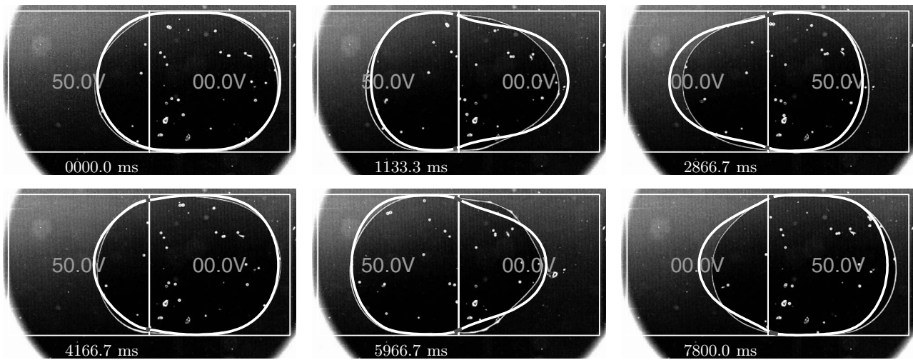
FIG. 9. Moving glycerin droplet experimental results with simulation overlay. The solid curve represents the simulated droplet boundary with small grayed regions (near the electrode edge) denoting pinned portions of the boundary. Frames show video snapshots of the experiment (experimental data courtesy of C. J. Kim and Jian Gong at UCLA). The applied voltage (50 V) switches between the left and right electrodes every 2 s. Each electrode is square with a side length of 1.5 mm. Simulation and device parameters are given in Table III. Note the large time scale because glycerin is highly viscous. The simulation follows the experiment fairly well, except there is some lagging in the “tail” region (enhanced online). [URL: http://dx.doi.org/10.1063/1.3254022.1 ]
