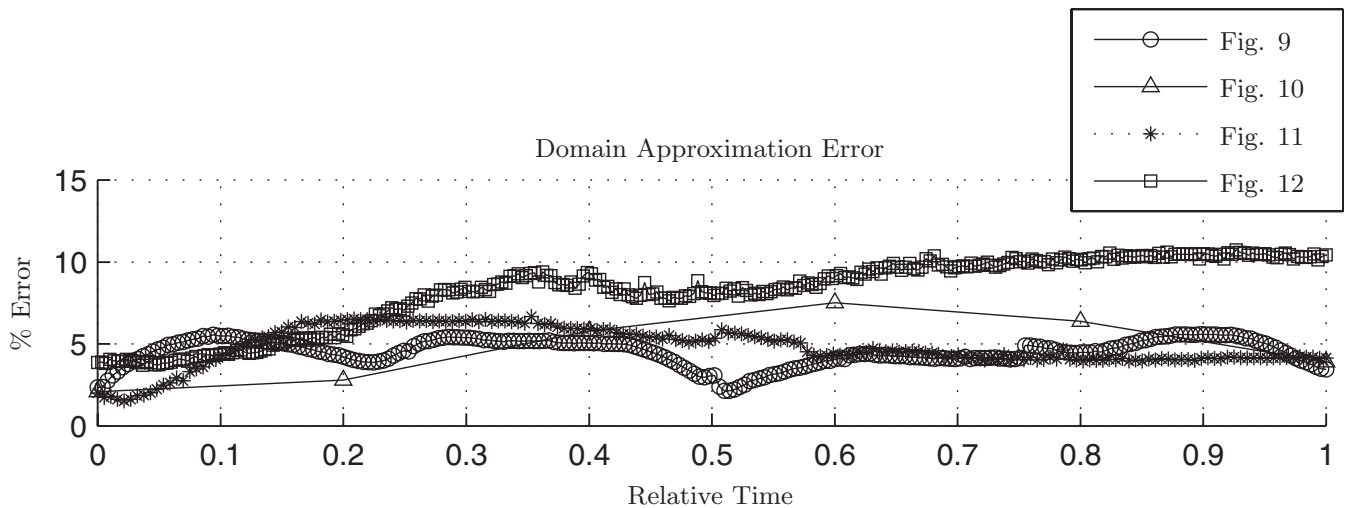
FIG. 8. Error between experimental droplet shape and simulated shape vs normalized time for all experiments. The error was measured using Eq. (39). Not all experiments have the same number of video frames (i.e., the experiment corresponding to Fig. 10 has only six video frames for the whole experiment). The overall error is reasonable. We also measured the frame-to-frame error for all experiments except Fig. 10. The frame-to-frame error is defined as the difference, via Eq. (39), between the extracted polygonal representation of the experimental drop in consecutive video frames. The average frame-to-frame error (over each experiment) for extracting a polygonal representation of the experimental droplet boundary is less than 0.7%. The maximum frame-to-frame error is less than 2%.
