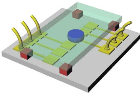
FIG. 2. (Color online) Schematic of sample EWOD device (figure courtesy of C. J. Kim, UCLA and Sung Kwon Cho, University of Pittsburgh) (Refs. 2 and 21). This EWOD system consists of two parallel plates with the top plate (transparent) acting as a ground electrode and the bottom plate containing a grid of embedded electrodes. The bottom plate also contains an extra dielectric layer to enhance device performance (not shown). A single droplet is shown near the center, but there may be many droplets of arbitrary shape between the two plates. Note that the height of each droplet is small compared to its horizontal size (these droplets are very thin puddles).
