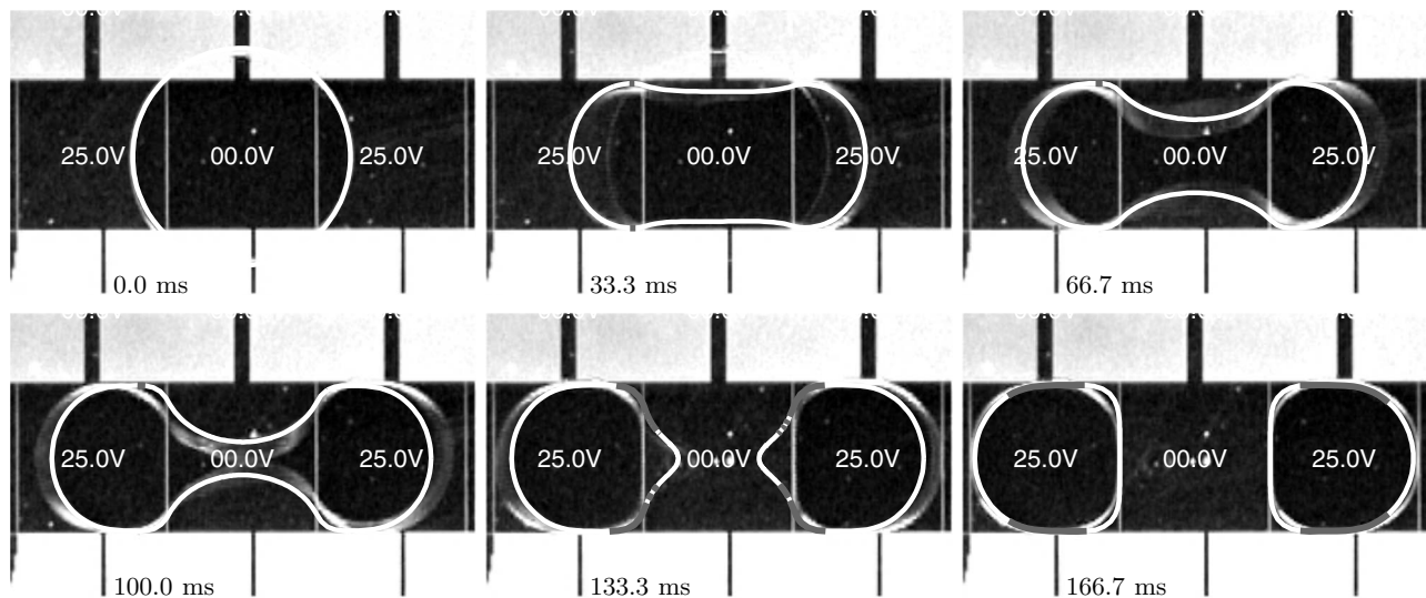
FIG. 10. Splitting water droplet experimental results with simulation overlay (solid curve is the simulation). Six frames show video snapshots of the experiment (experimental data courtesy of C. J. Kim and Sung Kwon Cho at UCLA) (Ref. 21). The three electrodes shown in each frame have activation voltages (from left to right) of 25, 0, and 25 V. Each electrode is approximately square with a side length of 1.4 mm. The gray regions of the simulated boundary indicate where the interface is pinned (i.e., cannot move in the normal direction). Only one parameter D_{\text{visc}} was fit to the simulation in order to match the time scale of the experiment.
