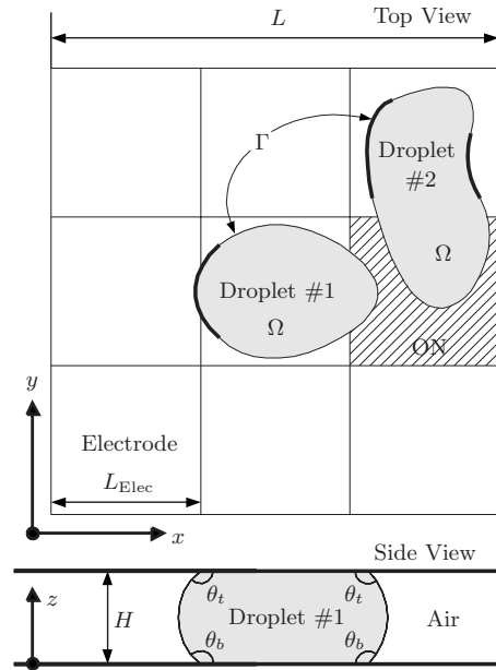
FIG. 3. Example EWOD device geometry (Ref. 2). The coordinate axes are defined such that the top and bottom plates of the device lie in planes parallel to the x - y plane. In this example, a 3 \times 3 grid of electrodes is shown, each with side length L_{Elec} , with one electrode active (the shaded square). Two liquid droplets are shown moving toward the active electrode to merge into one droplet. The domain of the liquid is denoted by \Omega and the liquid-gas interface is labeled \Gamma . The bold parts of \Gamma indicate “pinned” parts of the boundary due to contact line pinning. Note that only a subset of the boundary may be pinned; other parts may still move. A side view of the device is shown at the bottom (note: “droplet no. 2” is not shown here). The contact angles of the droplet, measured through the liquid, are denoted \theta_t and \theta_b (top and bottom). The physical parameters of the device, for each experimental setup, are listed in Tables I and III.
