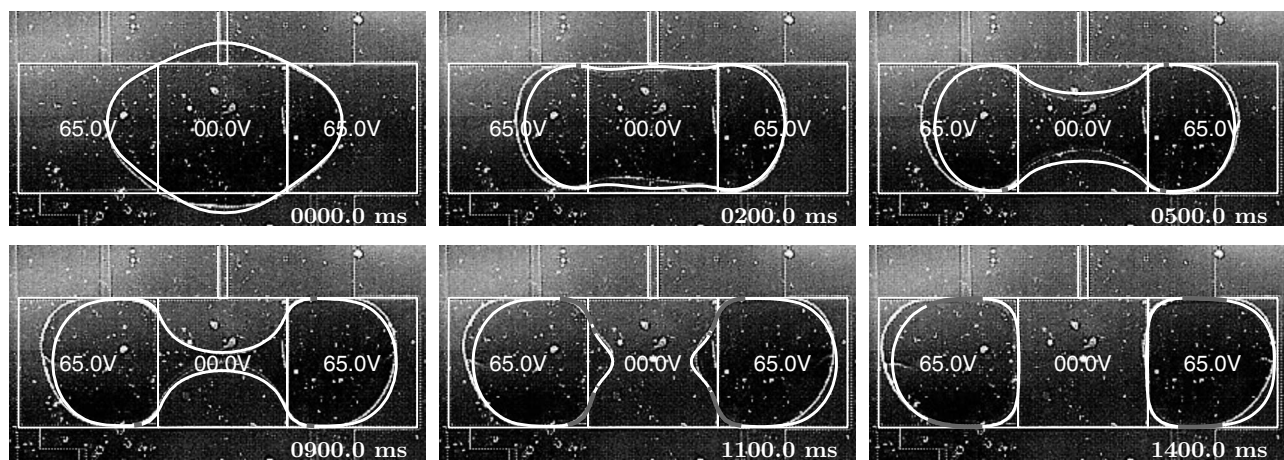
FIG. 11. Splitting glycerin droplet experimental results with simulation overlay (solid curve is the simulation). Frames show video snapshots of the experiment (experimental data courtesy of C. J. Kim and Jian Gong at UCLA). The applied voltage (65 V on the left and right electrodes) causes the droplet to be pulled apart and eventually split. Each electrode is approximately square with a side length of 1.5 mm. The match between the simulation and experiment is very good. In particular, note the relaxation of the interface immediately after pinchoff ( t=1100 ms). The only difference is that, in the experiment, slightly more fluid flows into the left satellite droplet than into the right droplet (as compared to the simulation). Also note the grayed regions of the boundary indicating pinned portions of the interface (enhanced online). [URL: http://dx.doi.org/10.1063/1.3254022.2 ]
