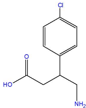
Baclofen chemical structure
