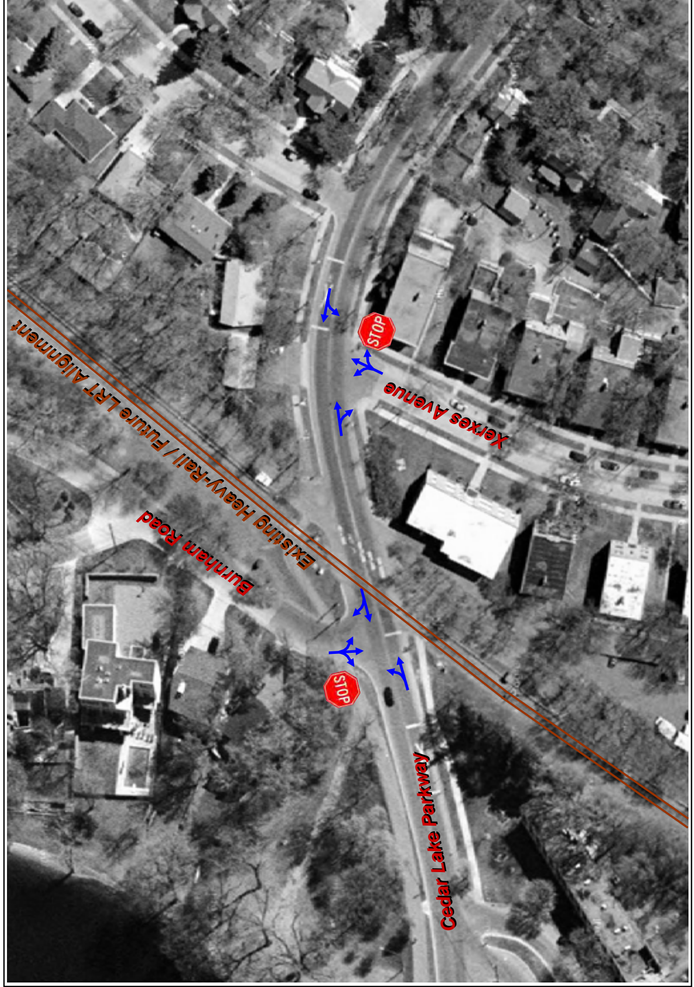
Figure 4 Existing Geometrics Potential Cedar Lake Parkway LRT Crossing
