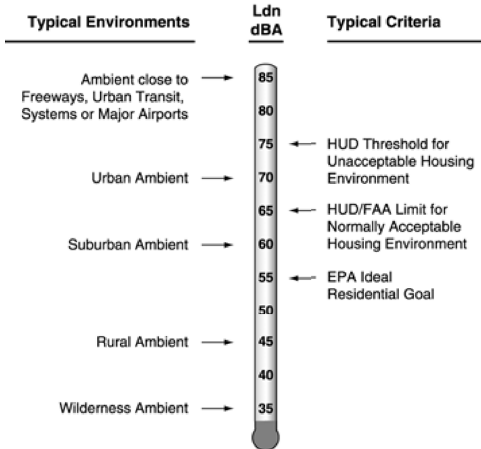
Exhibit 1. Examples of Typical Outdoor Noise Exposure
