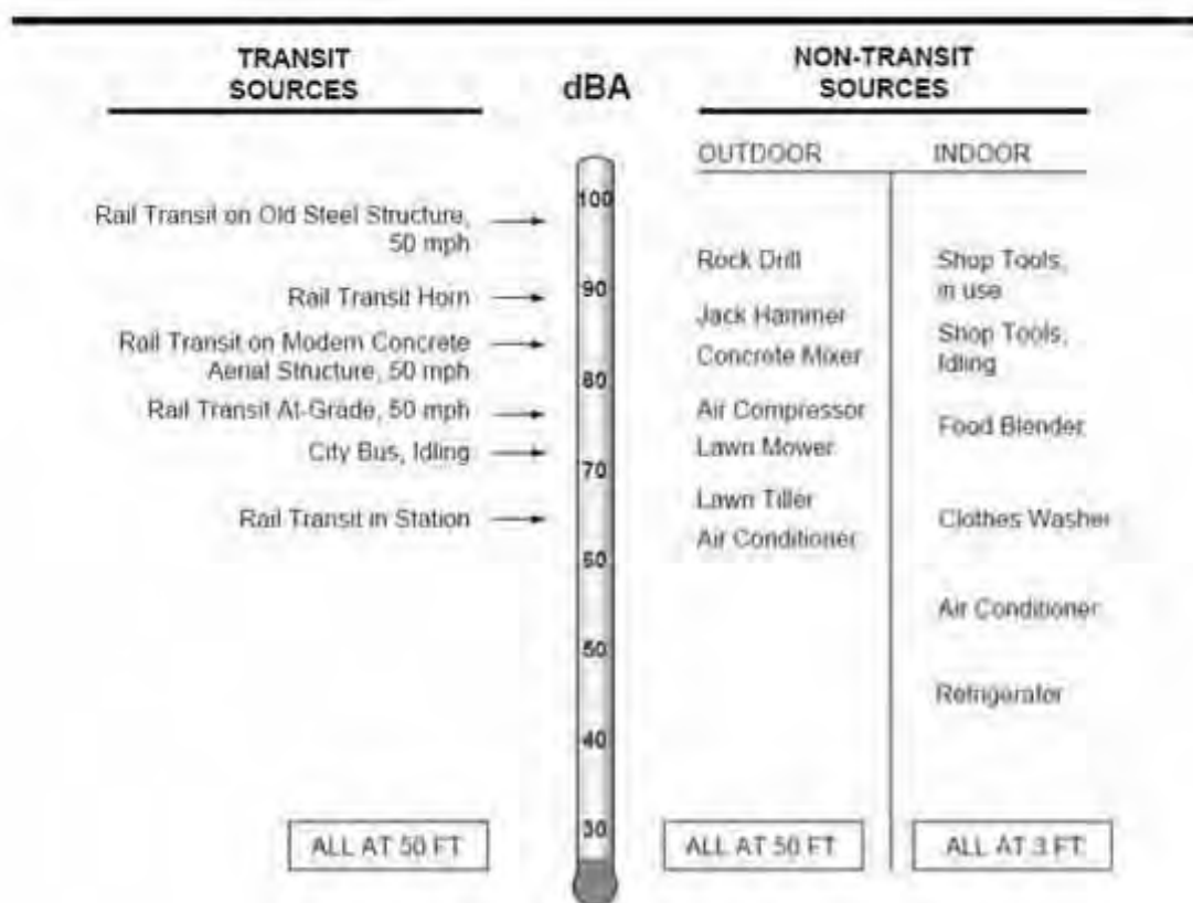
Figure 1. Typical A-Weighted Sound Levels
