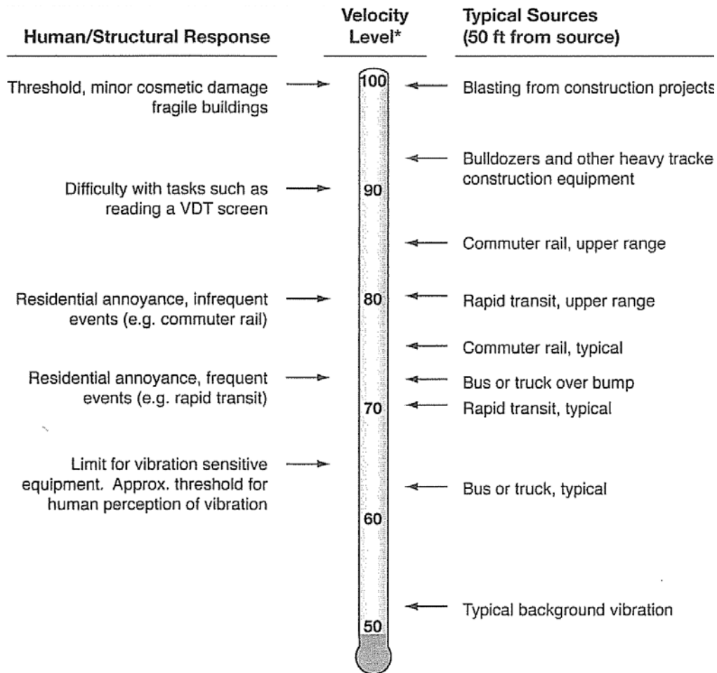
Figure 1. Common Vibration Sources
