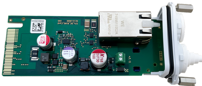
Fig. 21: S74 Network Slide in Board with RJ45 and VDC power supply
