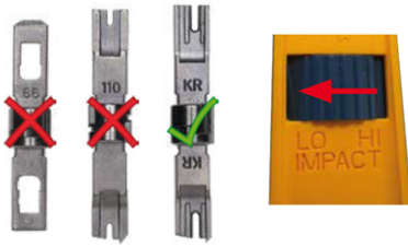
Fig. 16: LSA+/Krone tool set to LOW impact
