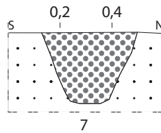
Befundtafel LA1_55 Profil Palisadenpfosten: 1: Pr_1261; 2: Pr_1263; 3: Pr_1277; 4: Pr_1267; 5: Pr_1268; 6: Pr_1274; 7: Pr_1275; 8: Pr_1276. M: 1:20.
