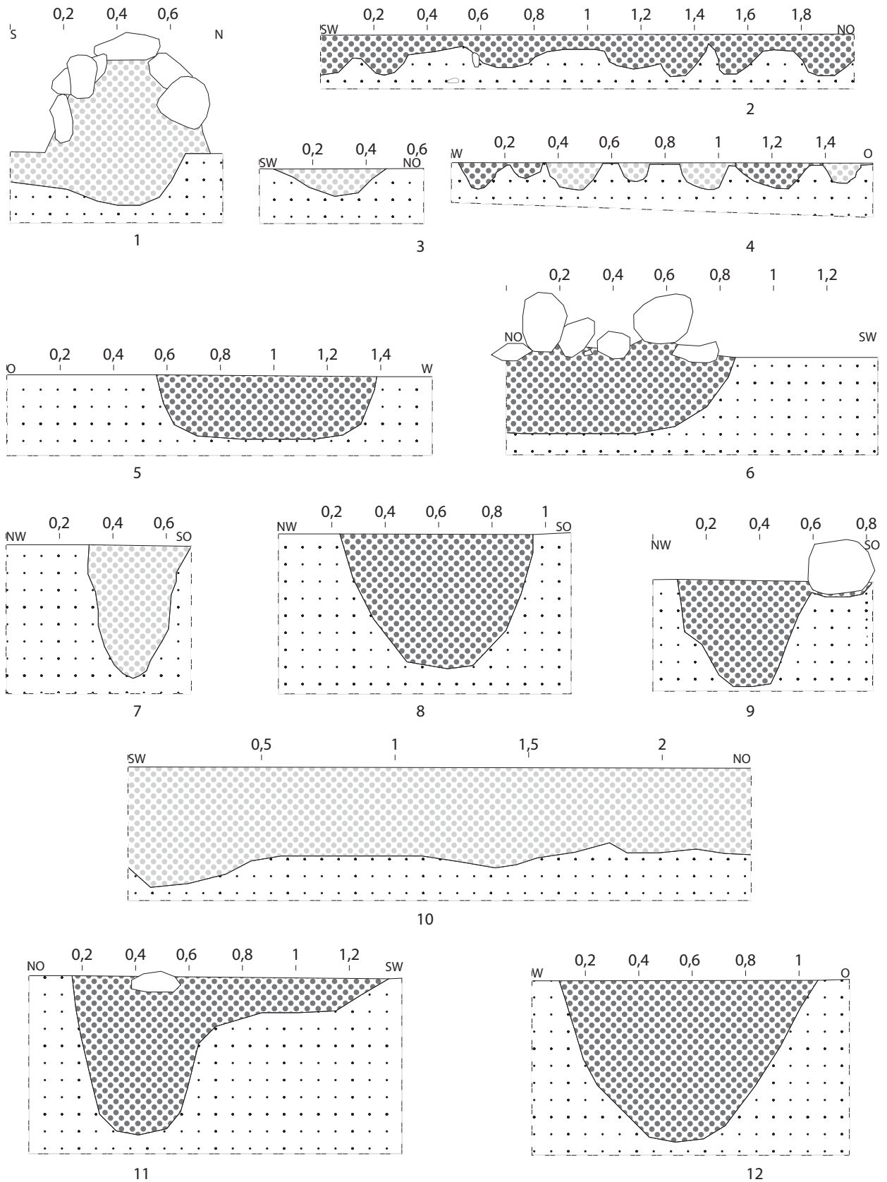
Befundtafel LA1_39 Profil Palisadengrübchen: 1: Pr_1564; 2: Pr_1303; 3: Pr_1557; 4: Pr_1462; 5: Pr_1302; 6: Pr_1298; 7: Pr_1311; 8: Pr_1296; 9: Pr_1304; 10: Pr_1310; 11: Pr_1523; 12: Pr_1530. M: 1:20.
