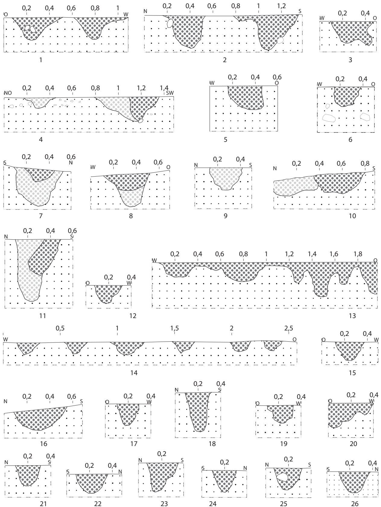
Befundtafel LA1_43 Profil Palisadenpfosten: 1: Pr_2; 2: Pr_3; 3: Pr_4; 4: Pr_5; 5: Pr_7; 6: Pr_8; 7: Pr_15; 8: Pr_16; 9: Pr_54; 10: Pr_55; 11: Pr_67; 12: Pr_76; 13: Pr_79; 14: Pr_80; 15: Pr_183; 16: Pr_184; 17: Pr_185; 18: Pr_186; 19: Pr_187; 20: Pr_555; 21: Pr_556; 22: Pr_557; 23: Pr_558; 24: Pr_559; 25: Pr_560; 26: Pr_561. M: 1:20.
