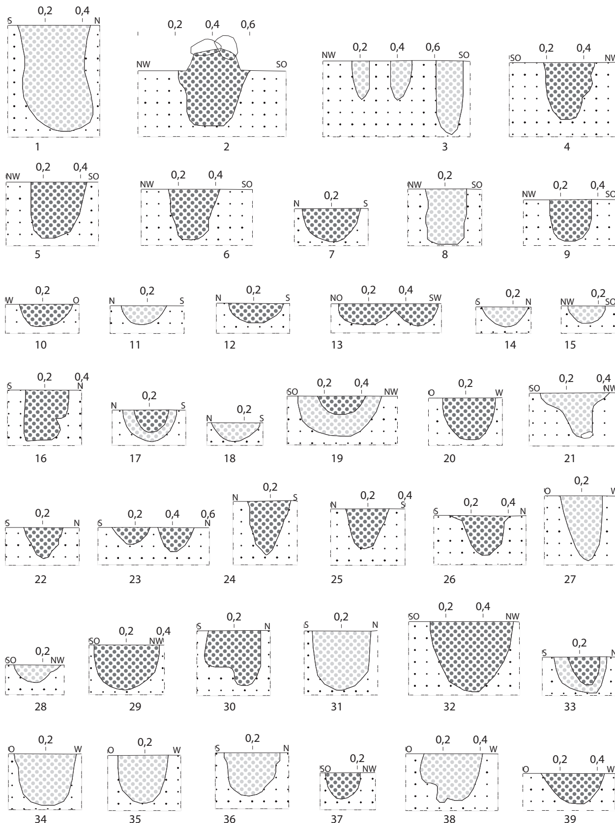
Befundtafel LA1_46 Profil Palisadenpfosten: 1: Pr_832; 2: Pr_744; 3: Pr_811; 4: Pr_747; 5: Pr_748; 6: Pr_749; 7: Pr_803; 8: Pr_810; 9: Pr_746; 10: Pr_807; 11: Pr_808; 12: Pr_804; 13: Pr_805; 14: Pr_812; 15: Pr_813; 16: Pr_814; 17: Pr_815; 18: Pr_816; 19: Pr_817; 20: Pr_818; 21: Pr_819; 22: Pr_820; 23: Pr_821; 24: Pr_822; 25: Pr_823; 26: Pr_824; 27: Pr_825; 28: Pr_826; 29: Pr_827; 30: Pr_830; 31: Pr_831; 32: Pr_696; 33: Pr_833; 34: Pr_412; 35: Pr_823; 36: Pr_824; 37: Pr_825; 38: Pr_826; 39: Pr_827. M: 1:20.
