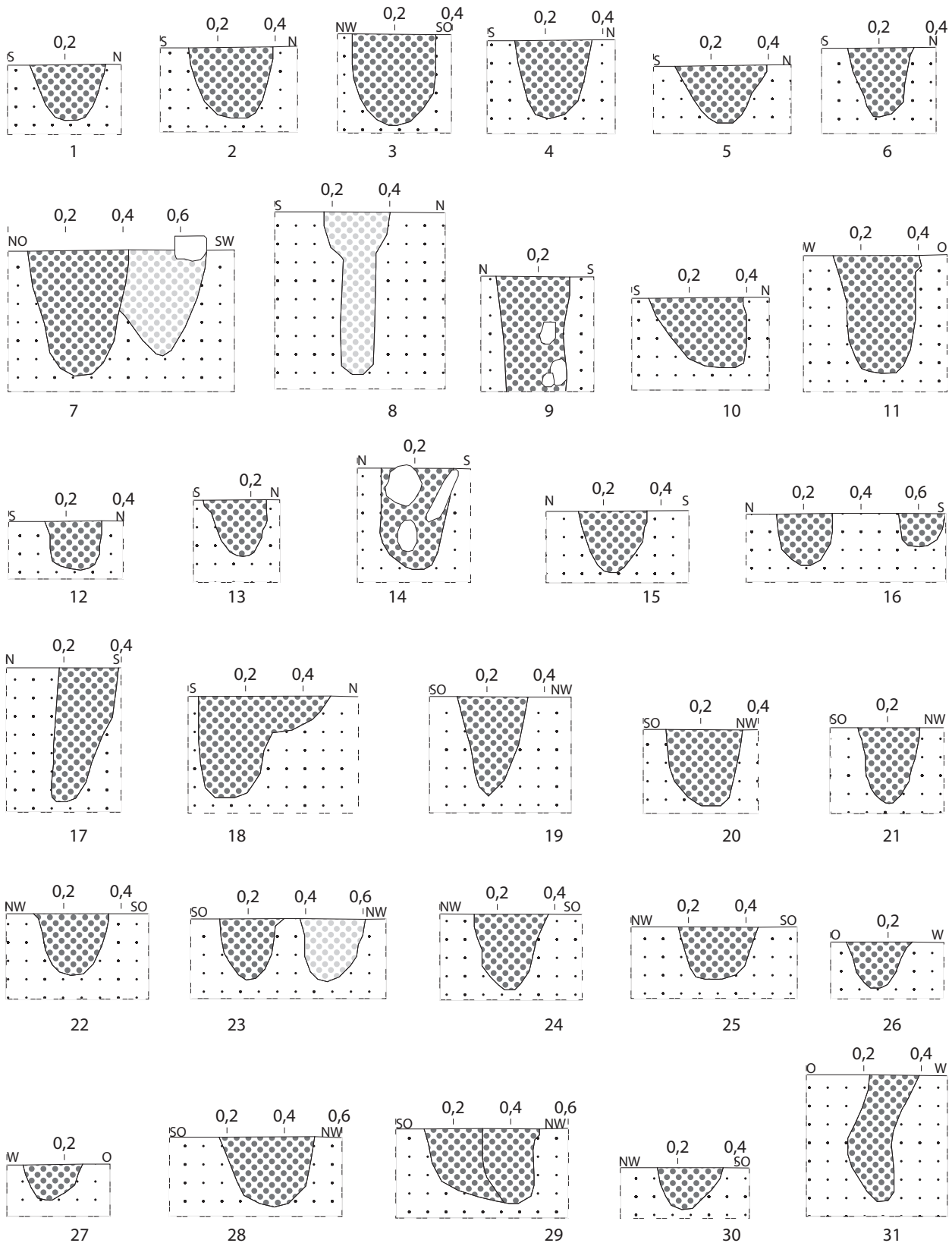
Befundtafel LA1_48 Profil Palisadenpfosten: 1: Pr_898; 2: Pr_899; 3: Pr_901; 4: Pr_902; 5: Pr_903; 6: Pr_904; 7: Pr_905; 8: Pr_906; 9: Pr_907; 10: Pr_908; 11: Pr_909; 12: Pr_910; 13: Pr_911; 14: Pr_912; 15: Pr_920; 16: Pr_921; 17: Pr_922; 18: Pr_923; 19: Pr_924; 20: Pr_925; 21: Pr_926; 22: Pr_927; 23: Pr_928; 24: Pr_929; 25: Pr_930; 26: Pr_931; 27: Pr_932; 28: Pr_933; 29: Pr_934; 30: Pr_935; 31: Pr_936. M: 1:20.
