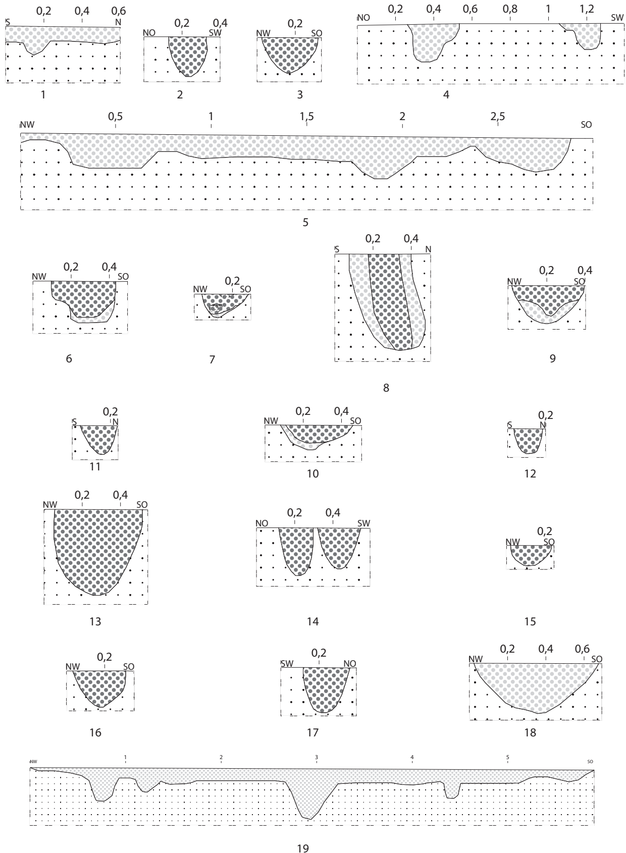
Befundtafel LA1_69 Profil Pfostenlöcher Haus 4: 1: Pr_519; 2: Pr_543; 3: Pr_522; 4: Pr_523; 5: Pr_526; 6: Pr_533; 7: Pr_520; 8: Pr_538; 9: Pr_539; 10: Pr_532; 11: Pr_540; 12: Pr_541; 13: Pr_542; 14: Pr_544; 15: Pr_545; 16: Pr_546; 17: Pr_548; 18: Pr_549; 19: Pr_550. 1-18 M: 1:20; 19 M: 1:40.
