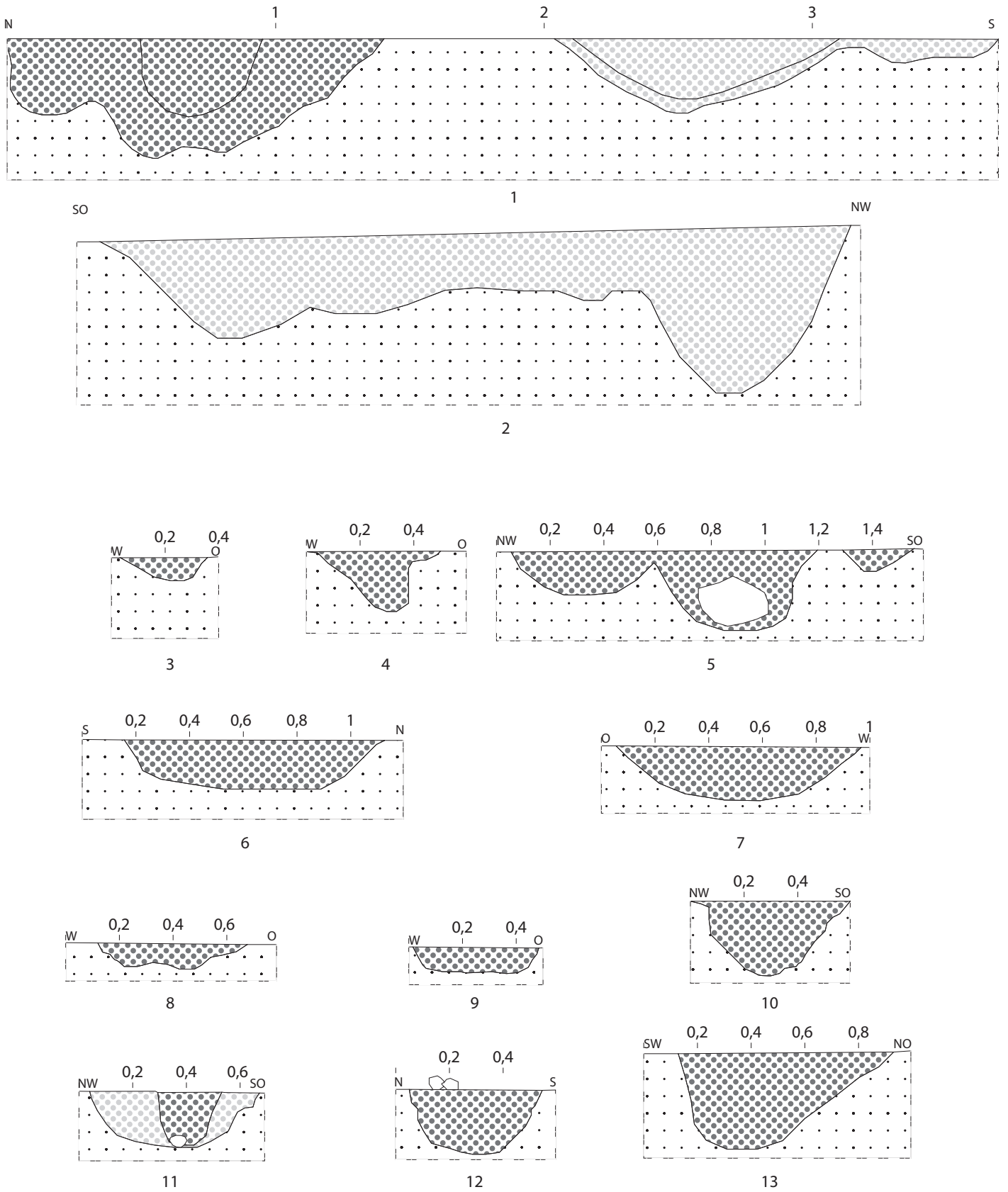
Befundtafel LA1_21 Profil Gruben: 1: Pr_448; 2: Pr_481; 3: Pr_565; 4: Pr_568; 5: Pr_566; 6: Pr_577; 7: Pr_578; 8: Pr_581; 9: Pr_582; 10: Pr_607; 11: Pr_594; 12: Pr_609; 13 Pr_612. M: 1:20.
