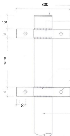
BACK SIDE ELEVATION DETAIL
