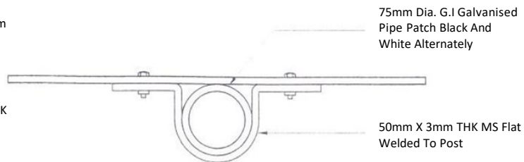
SECTION X-X
