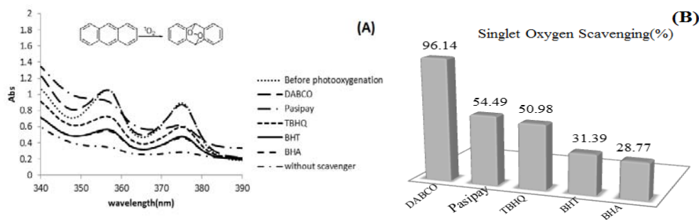
Fig1. Uv-vis spectra of anthracene photooxygenation with singlet oxygen in presence on different kind of singlet oxygen scavenger ( \lambda_{\text{max}}=375 nm ) after 5 min irradiation with air (1 atm) and 288 power LED lamps, 1 W, 2.3 V (59660LUX) (A), The scavenging capacity of different kind of singlet oxygen scavenger after 5 min irradiation with air (1 atm ) and 288 power LED lamps, 1 W,2.3 V(59660 LUX) (B).
