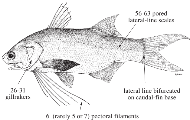
Fig. 81 Polydactylus approximans
