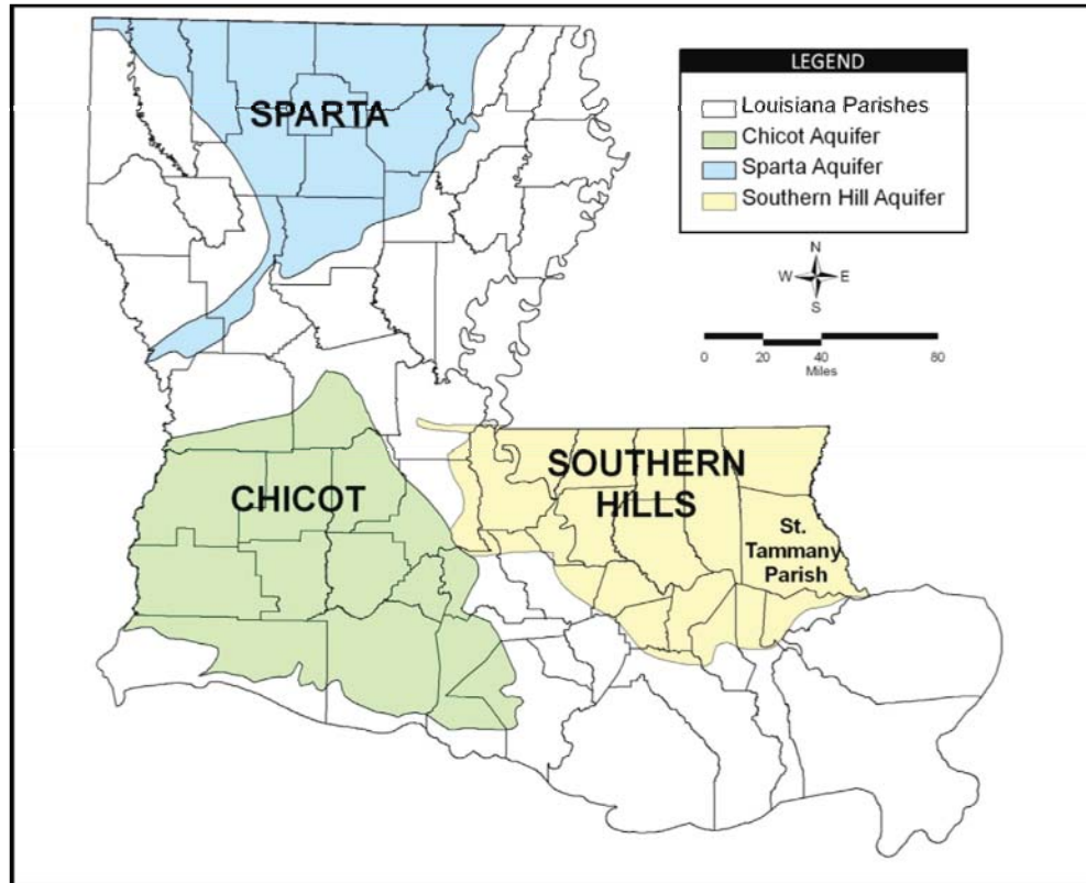
8 Figure 3-8. Major aquifers in Louisiana.
